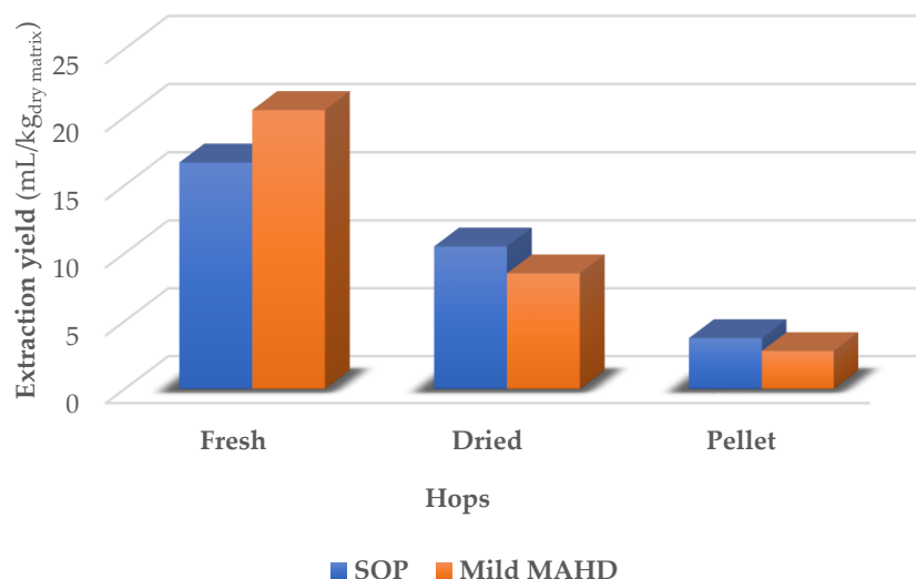
Figure 3. Volatile-fraction yield according to MAHD protocols.
