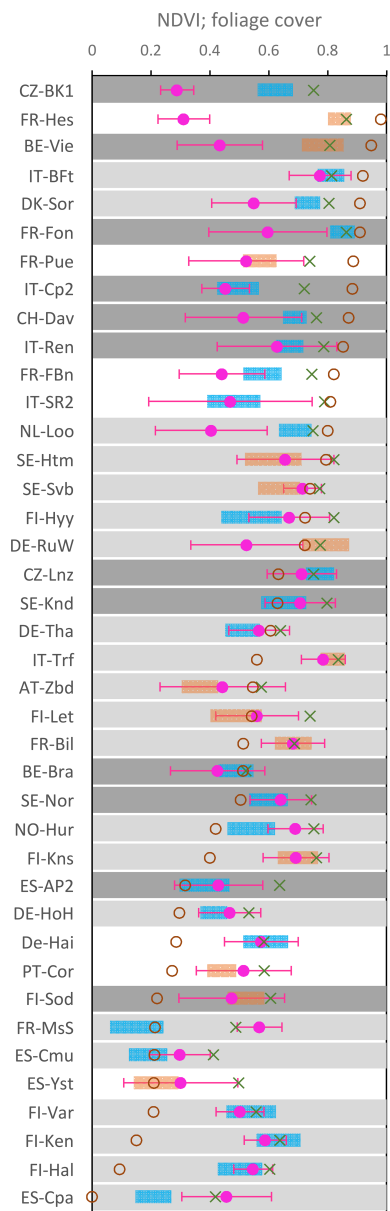
Figure 5. Estimated understory NDVI (NDVI u ) ranges for selected days (see Sect. 2.3 for how the ranges are obtained; blue bars – site-representative retrievals; orange bars – possible non-site-representative retrievals), in situ measurements (mean \pm 1 standard deviation (SD) shown in purple), and computed nadir total (understory and overstory) NDVI values from MODIS BRDF/albedo data (green crosses). The fraction of foliage cover is shown with brown open circles. MODIS BRDF parameters with lower quality flags are indicated with light gray (QA = 1) or dark gray (QA > 1) bars. QA = 0 – best quality with full inversion; QA = 1 good quality with full inversion (including the cases with no clear-sky observations over the day of interest and those with a solar zenith angle > 70^\circ ); QA > 1 – lower quality magnitude inversion, using archetypal BRDF shapes (for details please see Schaaf et al., 2002).
