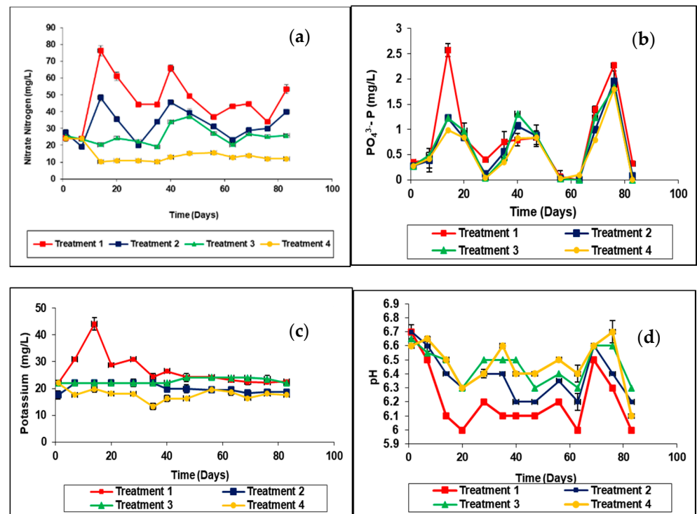
Figure 5. (a) Variation of \text{NO}_3^- -N with time; (b). Variation of \text{PO}_4^{3-} -P with time; (c). Variation of \text{K}^+ with time; (d). Variation of pH with time in the leaching column experiment.
