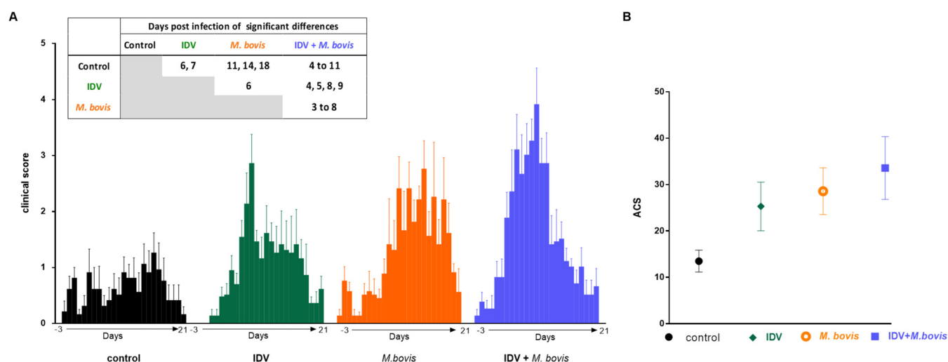
FIG 2 The coinfection increases the clinical scores. (A) Mean clinical scores with significant differences between groups. (B) Mean accumulated clinical score (ACS) for each group.
