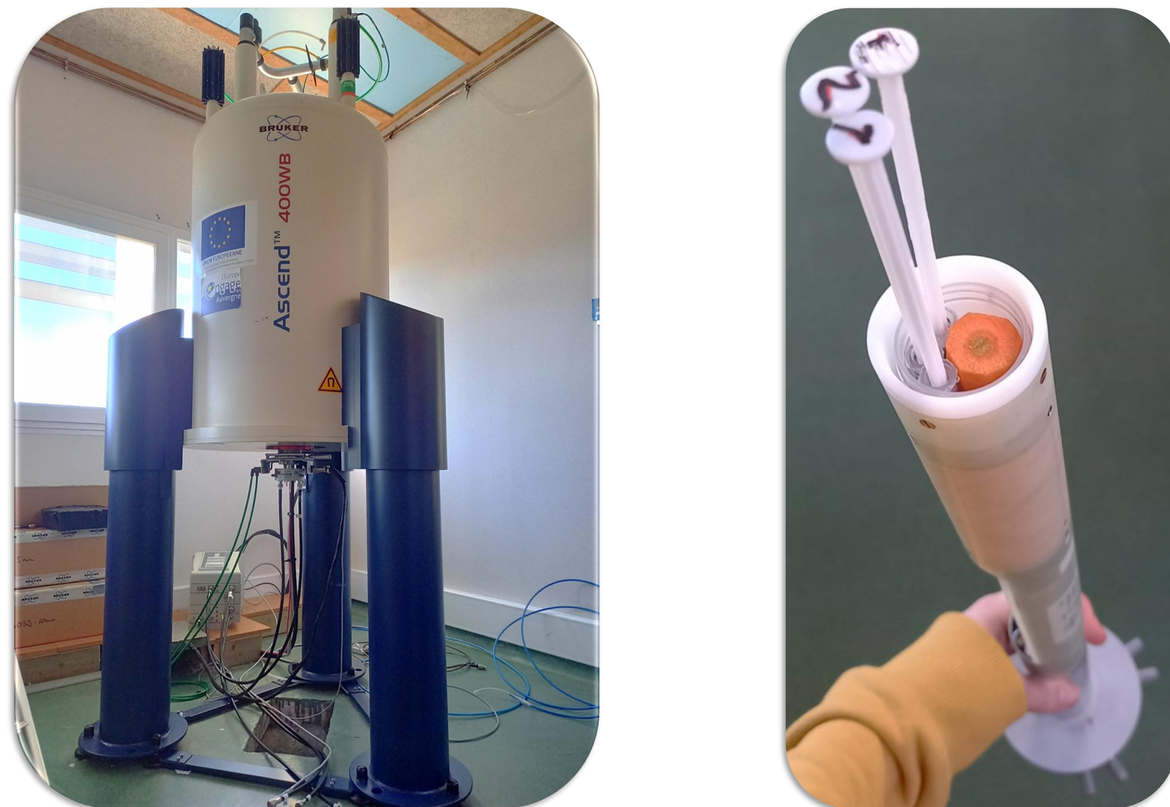
Fig 1: Picture of the equipment (Bruker Ascend 400WB with a Ø 3mm 1H/23Na volume radiofrequency antenna) and the set-up of a sample in the radiofrequency antenna.
