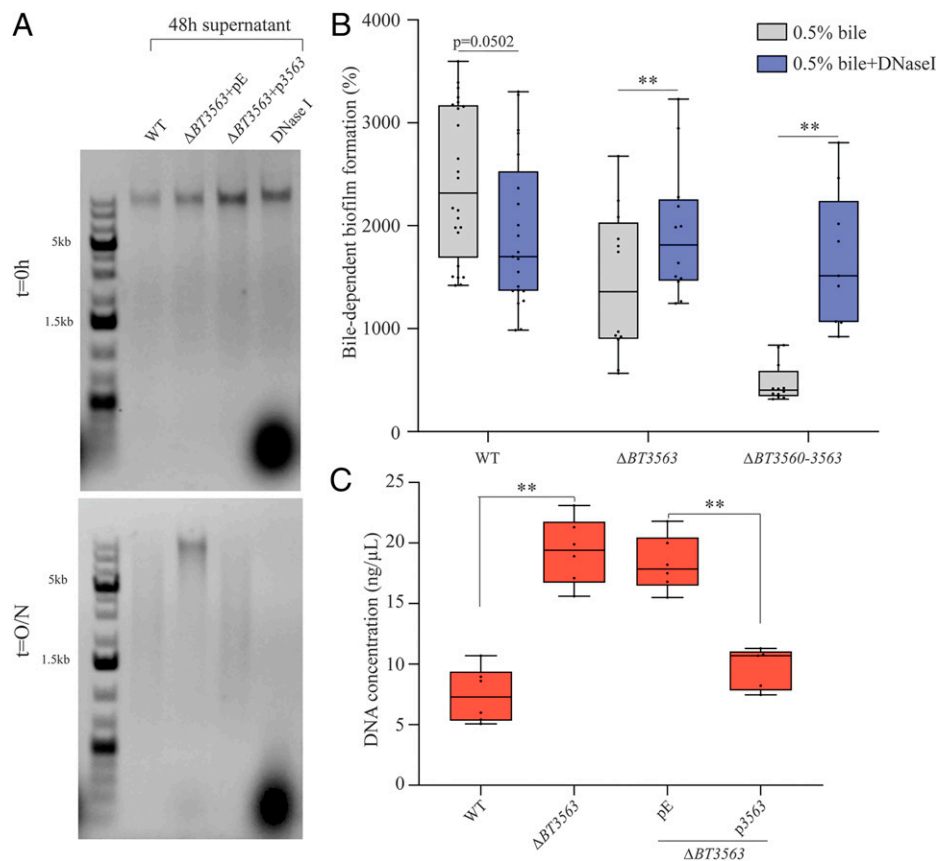
Fig. 3. BT3563 degrades nucleic acids in the extracellular matrix of bile-dependent biofilms. (A) Incubation of B. thetaiotaomicron genomic DNA (23 \mu\text{g} final concentration) with the supernatant of 48-h bile-free cultures, as indicated, and loaded immediately on a 1% agarose gel ( t = 0 h) and after an overnight incubation at 37^\circ\text{C} ( t = \text{O/N} ). A control using DNase I rather than supernatant is shown in the last lane. pE, empty vector; p3563, vector constitutively expressing BT3563. (B) A 96-well plate crystal violet biofilm assay after 48-h growth in BHIS + 0.5% bile extract, with or without DNase I. Mean of WT in BHIS is adjusted to 100% (not represented). Min-max boxplot of 9 to 21 biological replicates for each strain, each replicate is the mean of two technical replicates. **P value <0.005 , Wilcoxon matched-pairs signed rank test. (C) Extracellular DNA concentration ( \text{ng}/\mu\text{L} ) in the purified extracellular matrix of bile-dependent biofilms grown in BHIS + 0.5% bile extract for 48 h. Min-max boxplot of 6 biological replicates for each strain. **P value <0.005 , Mann-Whitney U test. pE, empty vector; p3563, vector constitutively expressing BT3563.
