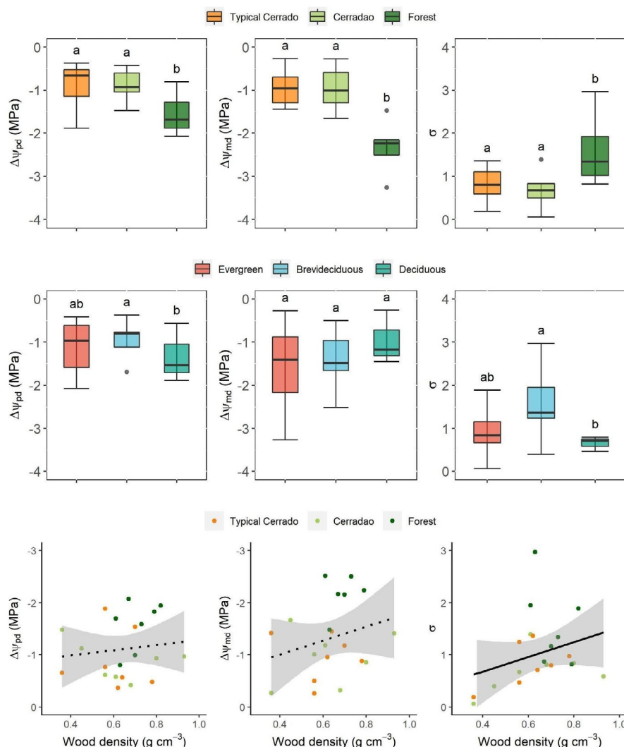
FIGURE 4 Comparison between the variation of \Psi_i at predawn ( \Delta\Psi_{pd} ); and variation of \Psi_i at midday ( \Delta\Psi_{md} ) and the slope angle ( \sigma ) of the relationship between leaf water potential at predawn ( \Psi_{pd} ) and midday ( \Psi_{md} ) for the different vegetation types (typical cerrado [STC], cerradão [SCF], and semideciduous seasonal forest [SSF]), different phenological groups, and the relationship with wood density. Statistics are shown in Table 2. Boxplots showing median and 25° and 75° percentiles, and different letters show statistical differences between groups ( p < .05 ). Solid lines show significant relationships ( p < .05 )
