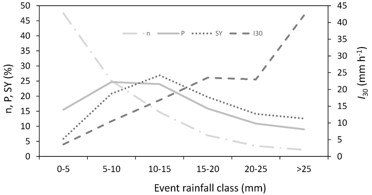
FIGURE 7 The percentage of the number of events ( n ), rainfall depth ( P , mm), sediment yield ( SY , \text{Mg ha}^{-1} \text{yr}^{-1} ) and average event maximum 30 minute intensity ( I_{30} , \text{mm h}^{-1} ) in the different event rainfall classes
