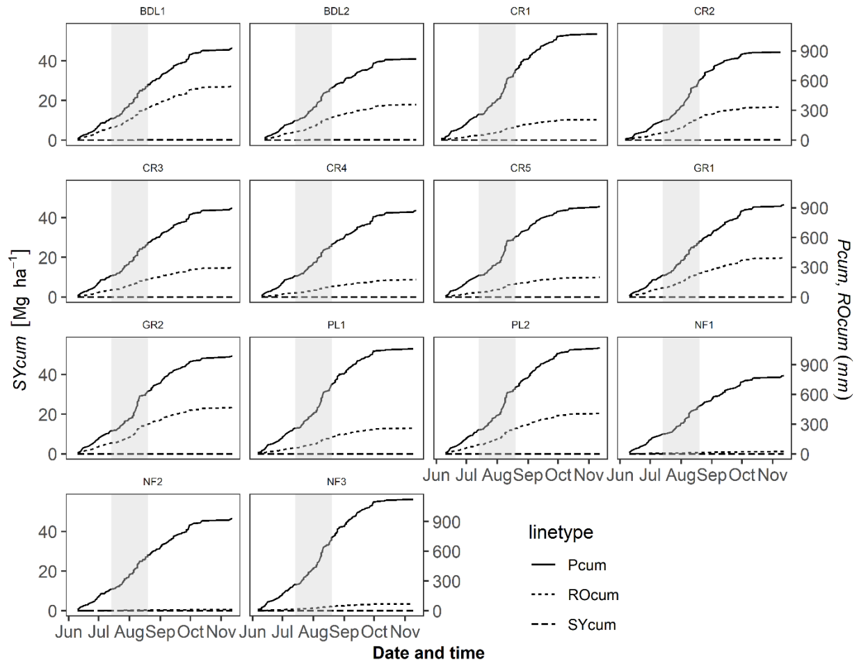
FIGURE 6 Cumulative event rainfall ( Pcum , mm), cumulative event runoff ( ROcum , mm), cumulative event sediment yield ( SY , \text{Mg ha}^{-1} ) for the different catchments (ID) of the 2019 rainy season (for more details see Table 1). Grey-shaded period indicates the steepest gradient in the curves
