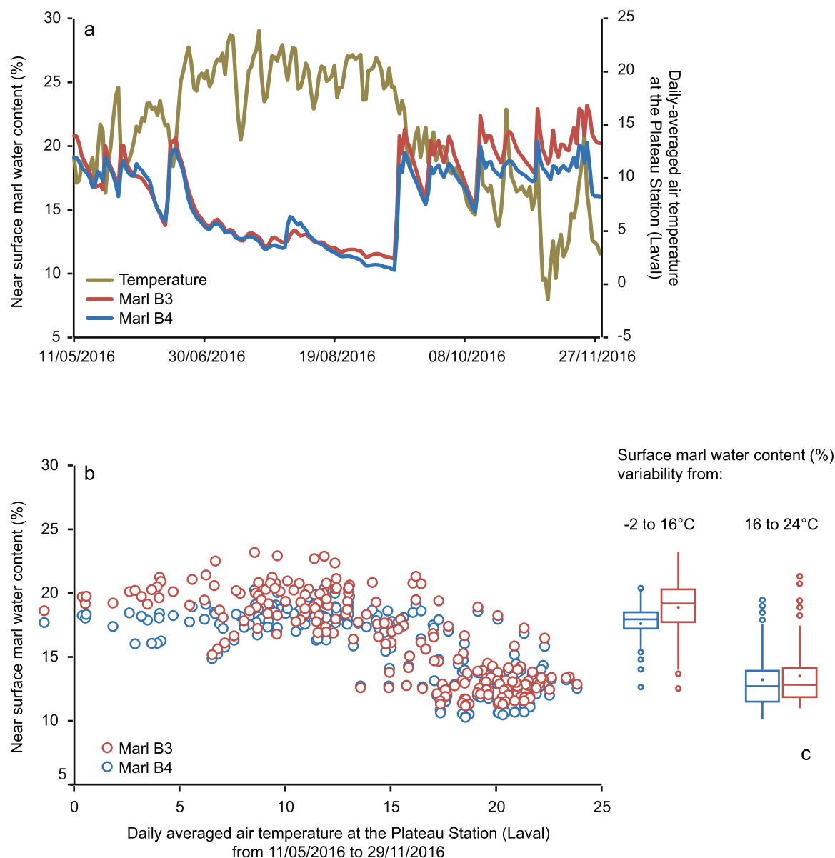
Extended Data Fig. 4 | The near surface water content of the Laval catchment (Draix, France) marls compared to the daily-averaged air temperature.
