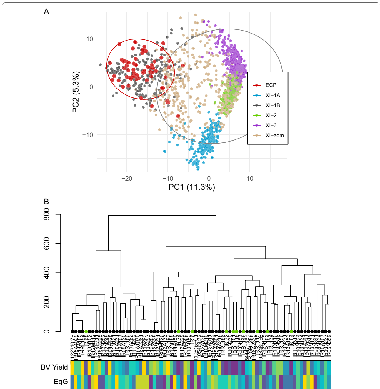
Fig. 6 Genotypic characterization of the elite core panel (ECP) based on genome-wide SNP markers. A Principal component (PC) analysis showing the grouping of ECP with Xian/indica (XI) group from the 3K-RG lines. B Dendrogram showing the relationship between ECP lines and with IRRI varieties (green dots). The heatmap at the bottom represents the breeding value for yield (BV Yield) and the equivalent complete generation (EqG) from the lowest (purple) to the highest (yellow) deciles
