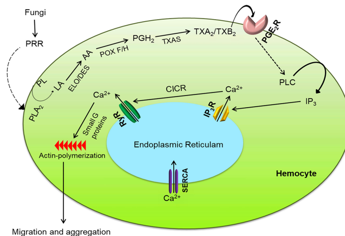
FIGURE 9 | Intracellular immune signaling in S. exigua hemocytes following fungal infection. Fungal hyphae or conidia are recognized by pattern recognition receptor ('PRR'), which activates the Toll pathway to increase PLA 2 activity. The activated PLA 2 releases linoleic acid ('LA'), which is desaturated and elongated into arachidonic acid ('AA'). AA is then oxygenated by two peroxidases ('POX F/H') into PGH 2 , which is isomerized into TXA 2 /TXB 2 by TXA 2 synthase ('TXAS'). TXA 2 /TXB 2 is transferred out of the cell to bind with its GPCR ('PGE 2 R') and activate phospholipase C ('PLC'). PLC increases intracellular inositol triphosphate ('IP 3 ') concentrations which binds to its receptor ('IP 3 R') on endoplasmic reticulum, thereby releasing Ca 2+ into the cytoplasm. Ca 2+ triggers calcium-induced calcium release ('CICR') from a ryanodine receptor ('RyR'). The free Ca 2+ is a secondary signal to activate small G proteins for actin polymerization to facilitate hemocyte behavior.
