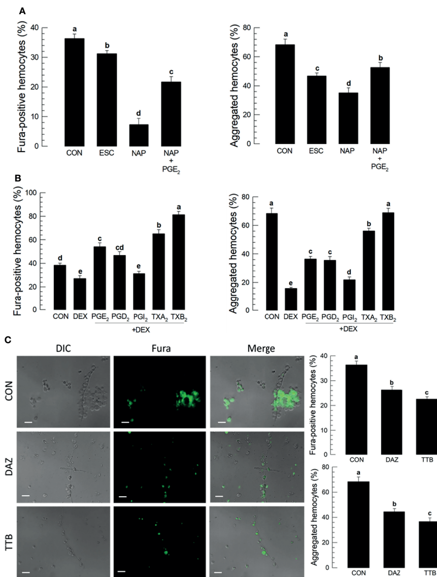
FIGURE 3 | Thromboxanes (TXA 2 and TXB 2 ) induce Ca 2+ signaling and hemocyte aggregation in S. exigua . Panel (A) reports that the COX inhibitor, NAP, but not LOX inhibitor, ESC, led to reduced proportions of Fura-positive hemocytes and reduced proportions of aggregated hemocytes. Co-injections with NAP+PGE 2 (1 μg/μL) rescued the influence of inhibiting COX. Panel (B) displays the influence of DEX on Ca 2+ signaling and hemocyte aggregation, which were reversed in larvae treated with DEX+the indicated prostanoids. Panel (C) shows the influence of the thromboxane biosynthesis inhibitor DAZ and the thromboxane receptor antagonist, TTB, on Ca 2+ signaling and hemocyte aggregation. The micrographs convey visual images, with reduced Fura signaling and the accompanying histograms show quantitative data with statistical analysis. Each treatment was replicated three times. Data analyzed and presented as described in Methods . Different letters above standard deviation bars indicate significant difference among means at Type I error = 0.05 (LSD test).
