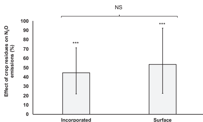
Fig. 1. Relative increase in field N_2O emission (mean \pm 95% CIs) with crop residues, as affected by residue placement. The number of observations and studies were 264 and 59 for incorporated, 75 and 21 for surface. *** indicates significance at p < 0.001 , and NS indicates not significant. Incorporated and surface applied crop residues increased N_2O emissions relative to the control (with the residues removed), whereas the difference between the two placement treatments was not significant.
