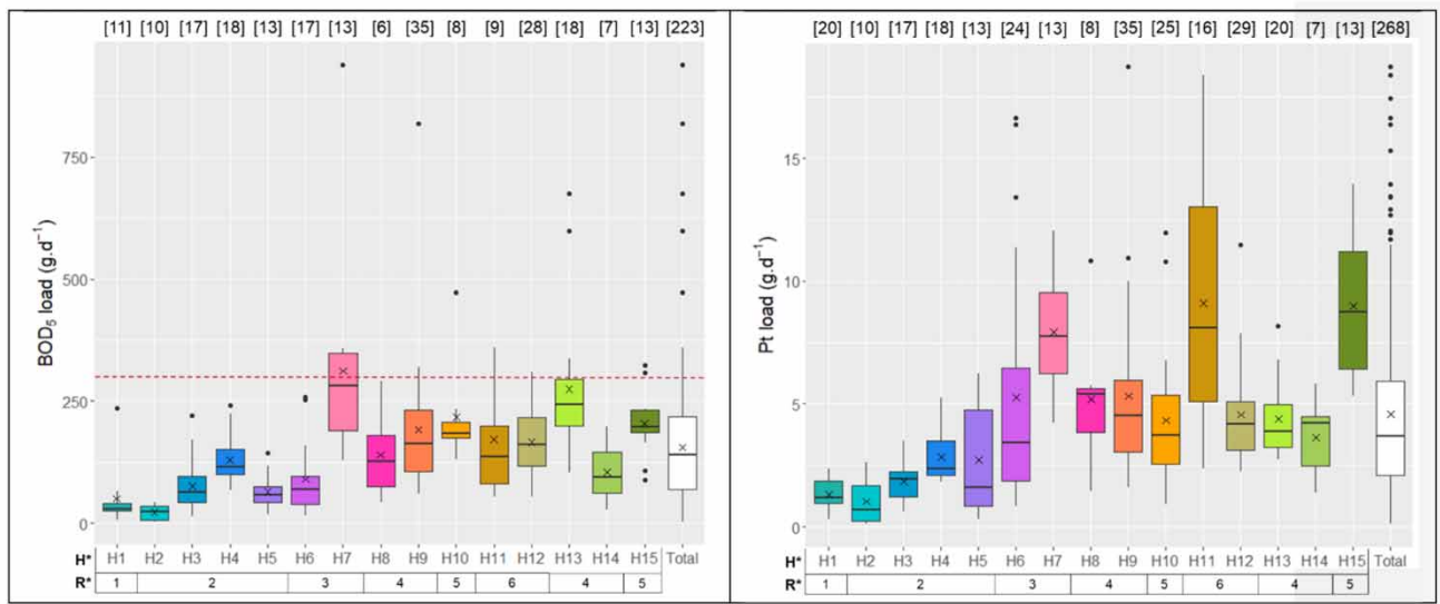
Figure 6 | Distribution of raw wastewater loads, in g \cdot d^{-1} , for 15 dwellings classified by increasing number of adult residents – left: BOD 5 ; right: TP. Note: H* = Household, R* = No. of residents. The number of data points in each dataset is in brackets; red dashes correspond to the rated load value of a household containing five occupants.
