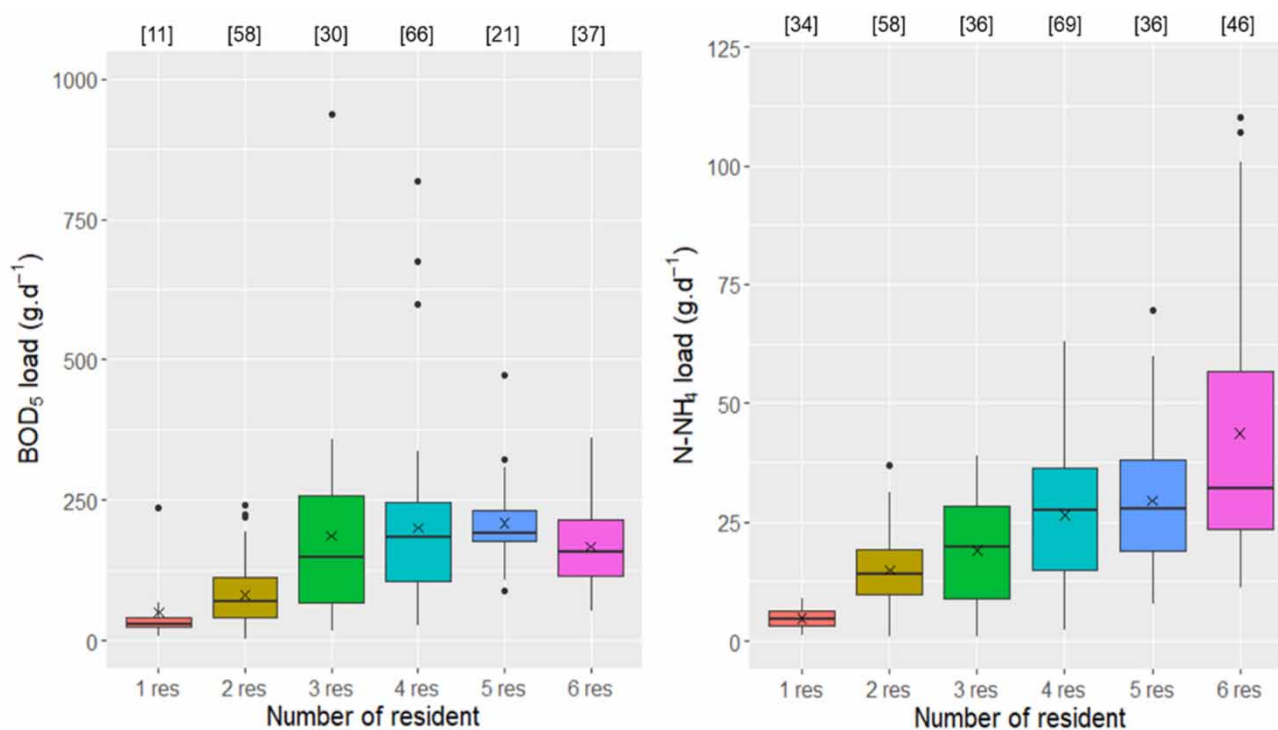
Figure 7 | Distributions of daily loads by number of residents, in BOD 5 (left) and NH 4 + -N (right).
