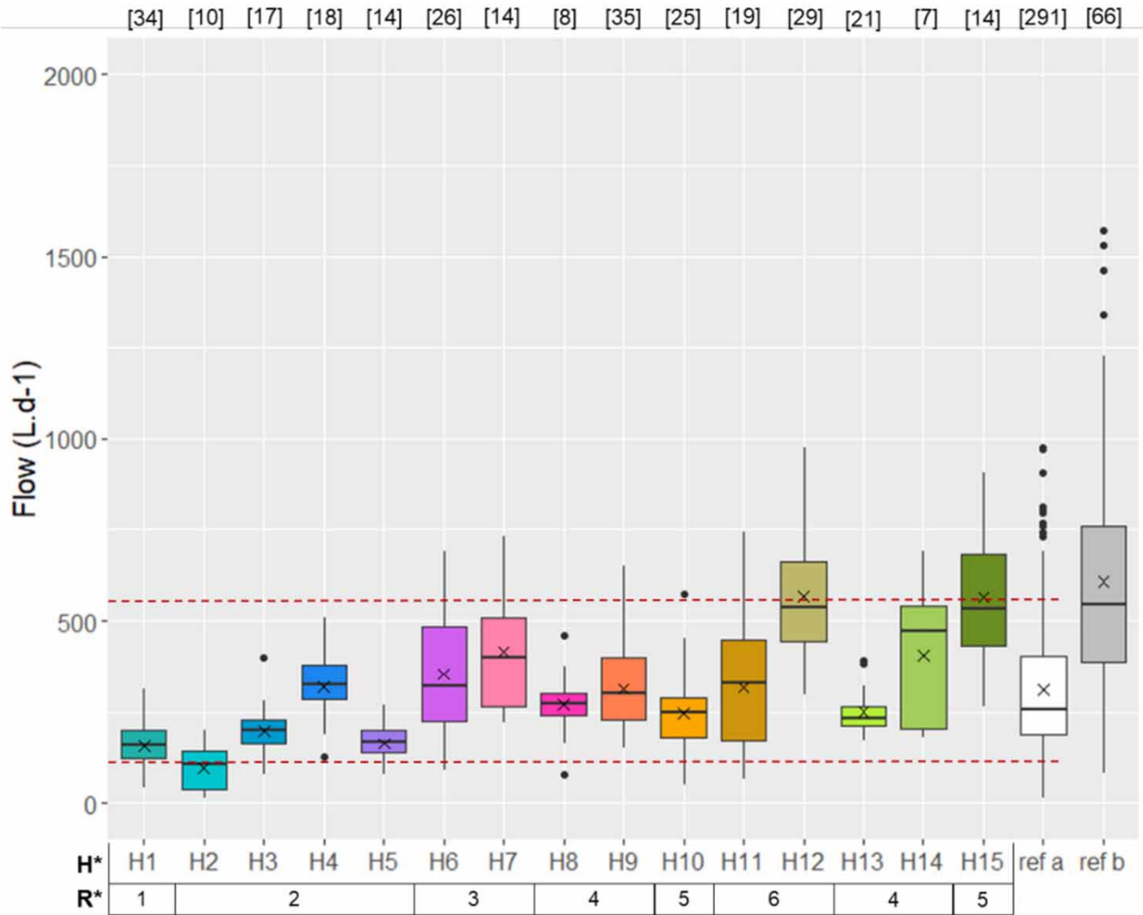
Figure 4 | Distribution of the daily volumes of 15 French households sorted by increasing number of adult residents and complete data for French (ref a) and American (ref b as per Lowe et al. 2009 ) datasets, in L.d^{-1} . Note: H* = Household, R* = No. of residents. The number of data points in each dataset is in brackets; red dashes correspond to the 10th and 90th percentiles of the complete French data distribution.
