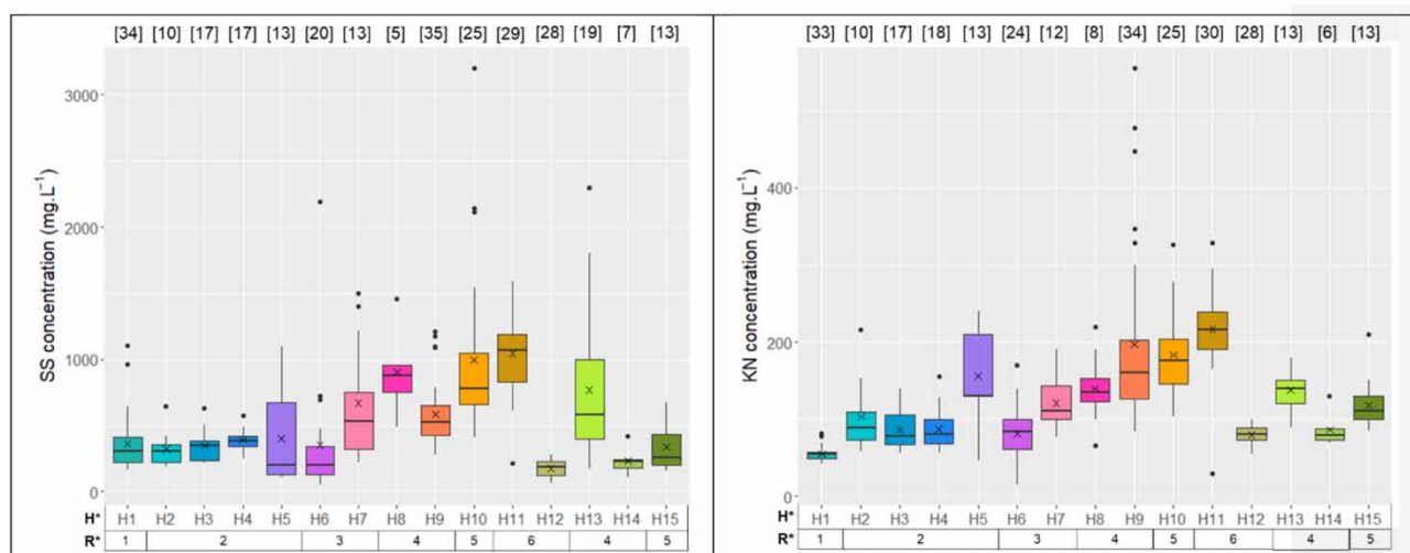
Figure 2 | Concentrations, in mg \cdot L^{-1} , of the raw wastewater from 15 dwellings – left: SS, right: KN. Note: H* = Household, R* = No. of residents. The number of data points in each dataset is in brackets.
