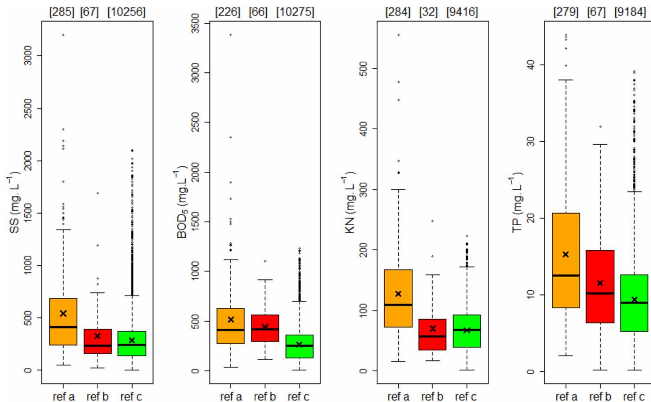
Figure 3 | Comparative distributions of raw wastewater concentrations, in mg.L -1 , from three datasets: [ref a] output by the present study, [ref b] reported by Lowe et al. (2009) , and [ref c] reported by Mercoiret (2010) . Note: The number of data points in each dataset is in brackets.
