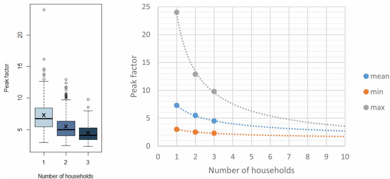
Figure 5 | Distribution of peak factor values vs. aggregated number of dwellings (left) and forecast of their evolution in average, minimum and maximum values (right).
