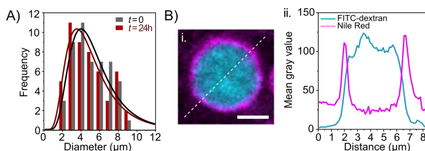
Figure 2. Fatty acid:fatty alcohol-stabilized all-aqueous emulsions. A) Distribution in the diameter of dextran-in-PEG droplets produced in the presence of sodium oleate (5 mM) and 1-decanol (15 mM) at t = 0 and after 24 hours, showing no change in the average size and polydispersity over time (number of droplets counted: 50). Size distributions were fitted using a log-normal function (shown as solid lines). B) Zoom of a single dextran-rich droplet stabilized by sodium oleate (5 mM) and 1-decanol (15 mM) at t = 24\text{h} (i) and associated fluorescence intensity line profile (ii, white dashed line in (i)), showing the homogeneous distribution of FITC-dextran throughout the droplet and the selective accumulation of Nile Red-doped fatty acid and fatty alcohol at the interface. False coloring to cyan and magenta were used for FITC-dextran and Nile Red, respectively. Scale bar, 2.5 \mu\text{m} .
