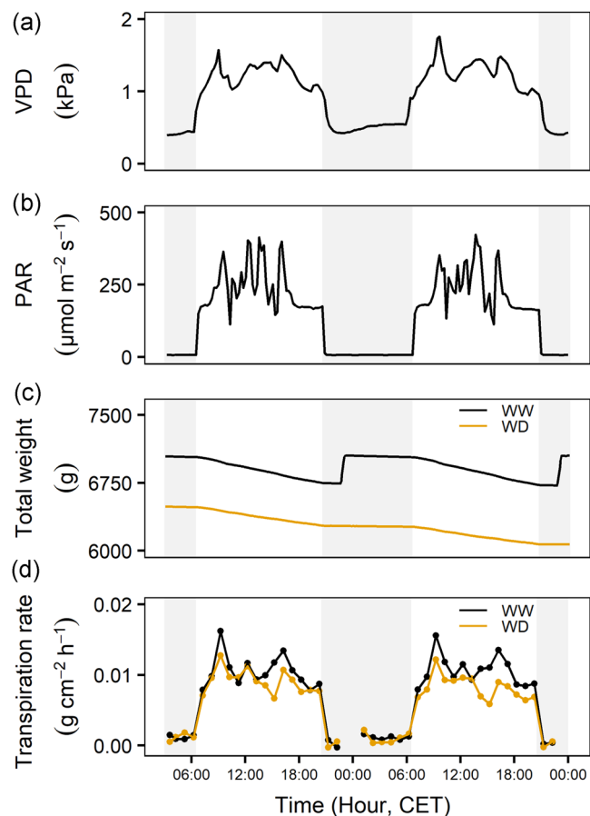
FIGURE 1 Time courses of (a) vapour pressure deficit (VPD), (b) photosynthetic active radiation (PAR), (c) raw weight measurements for a representative well-watered (WW) and water deficit (WD) plant of the Banksii_11 genotype and (d) calculated transpiration rates per unit leaf area. The transpiration rate was calculated every hour, the VPD, PAR and total weight are illustrated every 5 min. Grey areas indicate times of darkness [Color figure can be viewed at wileyonlinelibrary.com ]
