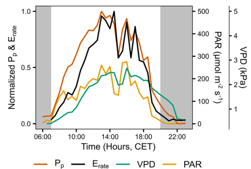
FIGURE 6 Diurnal dynamics of transpiration rate ( E_{\text{rate}} , black), leaf patch clamp pressure ( P_p , red), vapour pressure deficit (VPD, green) and photosynthetic active radiation (PAR, orange) of a representative well-watered plant of Musa acuminata ssp. malaccensis . The P_p values have been shown to be inversely coupled to the cell turgor pressure (Zimmermann et al., 2008). Grey areas indicate times of darkness [Color figure can be viewed at wileyonlinelibrary.com ]
