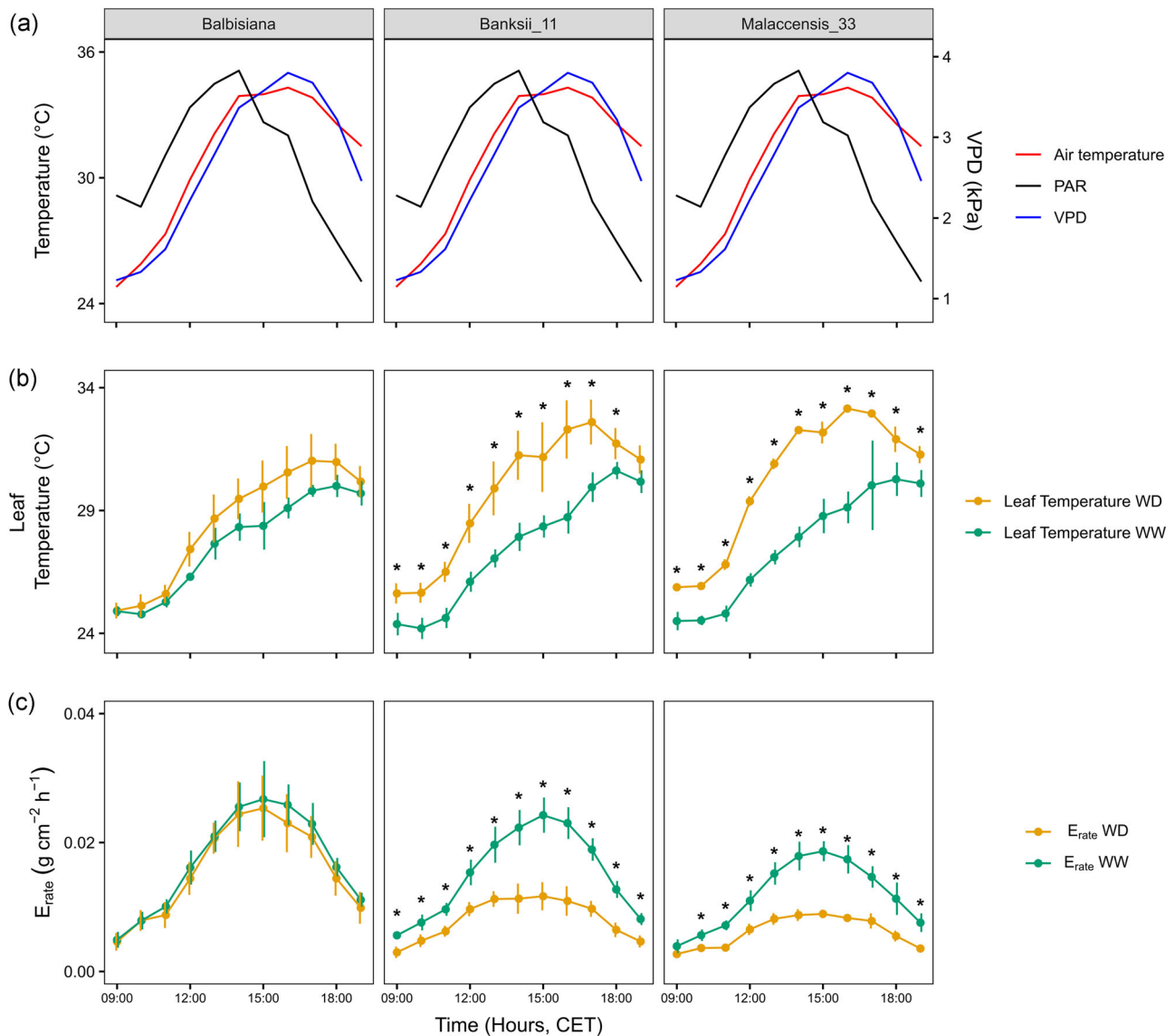
FIGURE 3 Environmental conditions, leaf temperature and transpiration rate for three wild banana genotypes during 1 day of the validation experiment. (a) Air temperature (red), photosynthetic active radiation (PAR; black) and vapour pressure deficit (VPD; blue) throughout the measurement day. (b) Leaf temperature development for well-watered (WW; green) and water deficit (WD; orange) plants. Data represent the mean \pm stdev ( n = 4 per treatment and genotype, * for p < 0.05 ). (c) Transpiration rate evolution of WW (green) and WD (orange) plants. Data represent the mean \pm stdev ( n = 4 per treatment and genotype, * for p < 0.05 ). [Color figure can be viewed at wileyonlinelibrary.com ]
