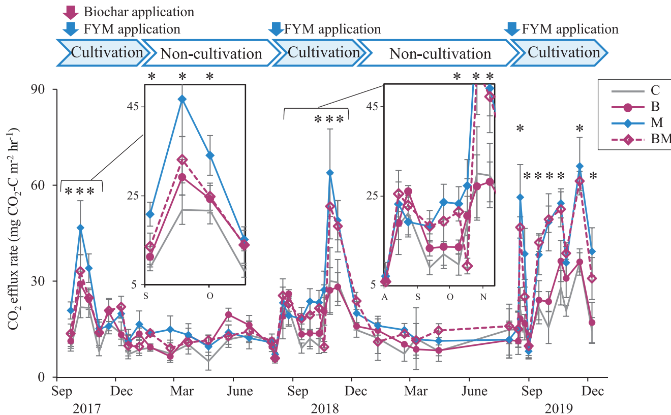
FIGURE 1 Seasonal variations in \text{CO}_2 efflux rate. C, control plot; B, biochar application plot; M, farmyard manure (FYM) plot; BM, biochar and FYM application plot. Bars present standard error. Stars represent significant differences among the treatments on each sampling date based on the Tukey-Kramer multiple comparison test ( p < 0.05 ) [Color figure can be viewed at wileyonlinelibrary.com ]
