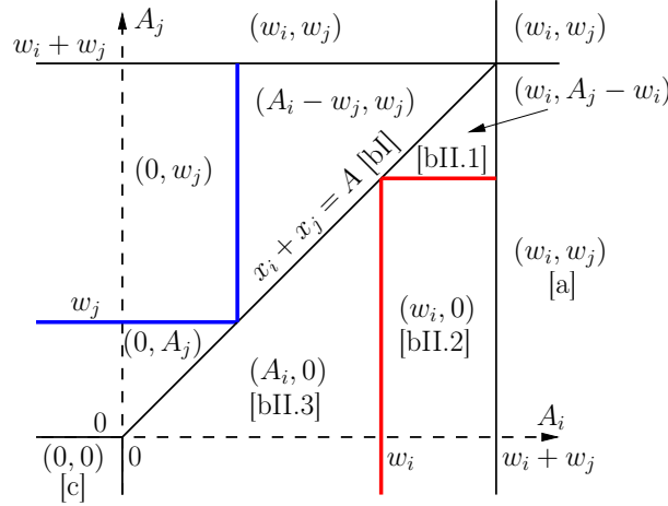
Figure 16: Nash equilibria as a function of (A_i, A_j)
