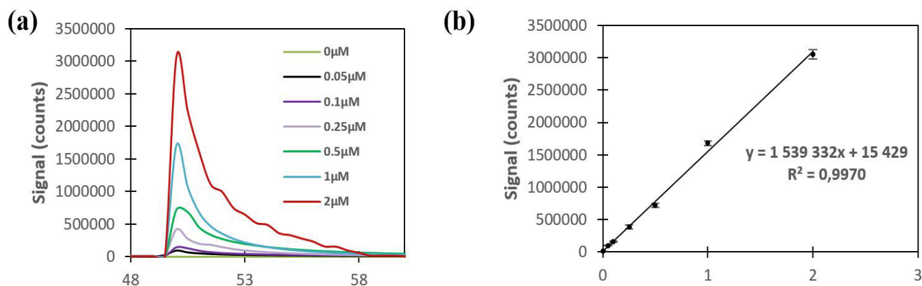
Figure 4. (a) ECL response obtained using BDD electrodes and optimised voltage pulse of solutions containing skatole over a concentration range (0, 0.05, 0.1, 0.25, 0.5, 1, 2 \mu M). The procedure used was 0 V (10 s) \rightarrow -1.8 V (40 s) \rightarrow 0.8 V. (b) The corresponding calibration plot for skatole using ECL peak height vs concentration ( n = 5 ).
