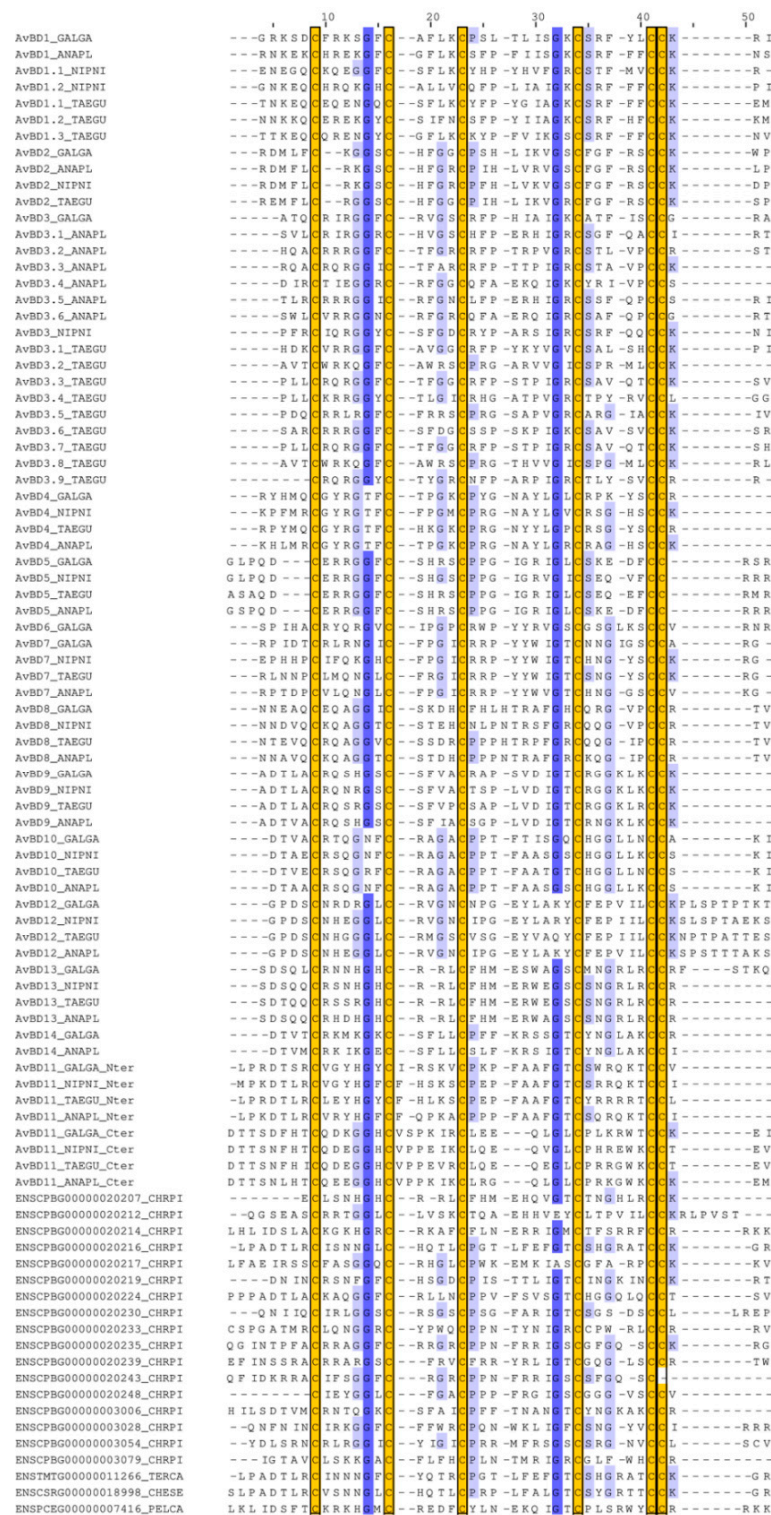
Figure 8. MSA of the N-terminal and C-terminal domains of AvBD11 with monodomain AvBDs and turtle \beta -defensins. MSA was performed with MAFFT and drawn with Jalview with a blue colour gradient (100% of identity for dark blue) and trimmed at each extremity to adjust to the length of the
