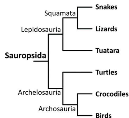
Figure 2. Cladogram of sauropsids. According to Crawford et al. [22] and Gemmill et al. [23].
