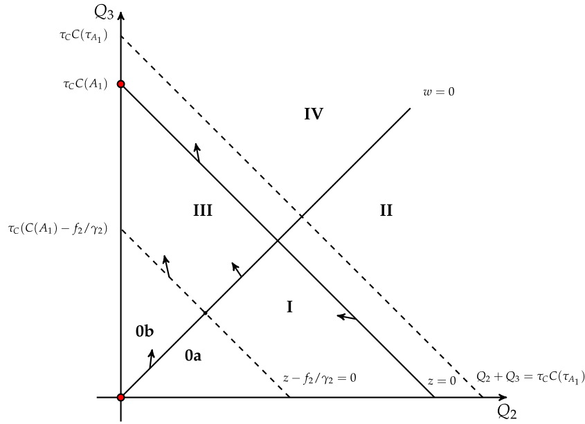
Fig. 7. Scheme of the vector field projected on the Q_2, Q_3 -plane.
