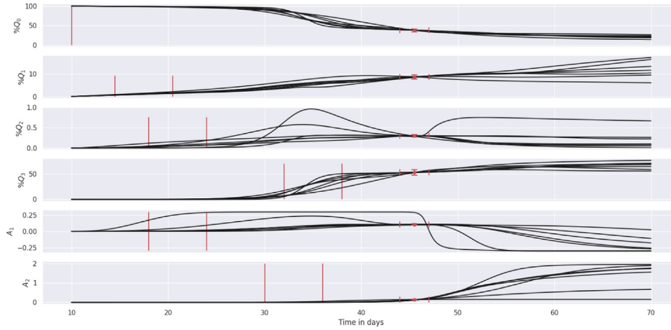
Fig. 3. Evolution of cell populations and axons in the pancreas for 7 different sets of parameters. The x-axis is the time in days. For the top four graphs, the y-axis corresponds to percentage of a specific population in the pancreas. The vertical red lines correspond to the time of appearance within a tolerance of six days. The red dots at day 45 correspond to the observation y^* for the mouse 1 (see Fig. 2) and the confidence intervals of the data are represented by the red segments. Each curve on the same graph is associated to its set of parameters (see Table 3). All sets of parameters have almost the same optimization score (under 10), however the dynamics are different. .
