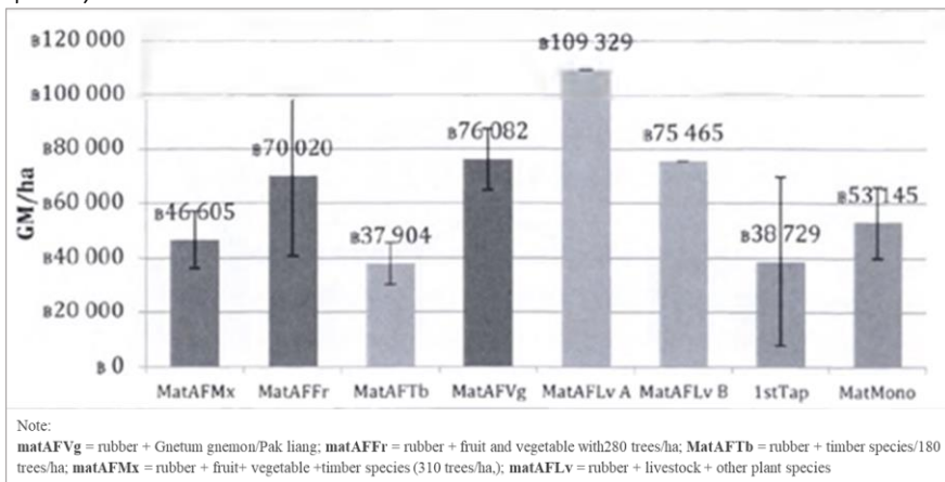
Figure 1. Gross margin per hectare and per year for different kinds of rubber agroforestry systems and comparison with rubber monocrops (Source: Stroesser, 2018)
