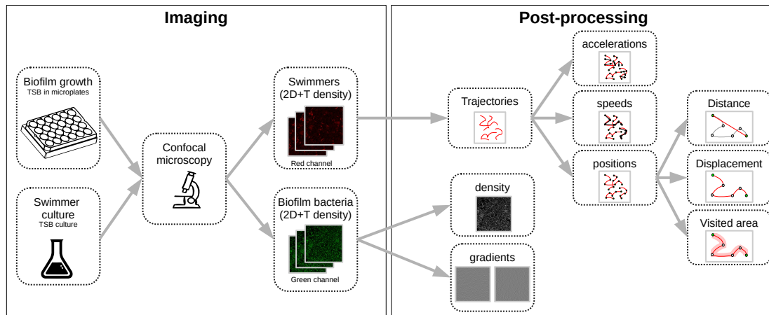
Figure 1: Microscopy data and model outlines. (a) Temporal stacks of 2D images are acquired, with different fluorescence colors for host bacteria ( Staphylococcus aureus , green) and swimmers ( Bacillus pumilus , Bacillus sphaericus or Bacillus cereus , red). Bacterial swimmers navigate in a host biofilm and are tracked in the different snapshots. Swimmer trajectories are represented with white lines. High density and low density zones of host cells are visible in the biofilm (green scale). (b) Additionally to speed and acceleration distributions, three trajectory descriptors are considered. Distance is the distance between the initial and final points of the trajectory. Displacement is the total length of the trajectory path. Visited area is the total area of the pores left by the swimmer during its path. Hence, when a swimmer retraces its steps, the displacement is incremented but not the visited area. (c) Three different mechanisms are considered in the mechanistic model. Biofilm-dependant speed . A target speed is defined accordingly to the local density of biofilm and asymptotically reached after a relaxation time. Biofilm-dependent direction . Swimming direction is defined accordingly to the local biofilm density gradient. Random walk . A Brownian motion is added. (d) The image acquisition workflow is composed of a first step at the wet lab where host biofilm and swimmer are plated and imaged in different color channels. Then a post-processing phase recomposes the swimmer trajectories with tracking algorithms. Then, temporal positions, speeds and accelerations are computed. On the biofilm channel, density and density gradient maps are processed at each time step.
