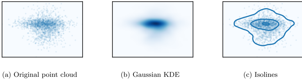
Figure A.8: Illustration of the Gaussian KDE isovalues computation. Starting from a random 2D point distribution, a gaussian KDE is computed using the scipy.stats function. Then, the gaussian KDE is evaluated at the original point positions, and quantiles of the resulting values are computed (quantiles 0.05, 0.5 and 0.95). Gaussian KDE isolines corresponding to this quantiles are finally computed. This isolines enclose respectively 5, 50 and 95 % of the points of the original distribution, centered in the densest area of the initial point cloud. This procedure gives a good representation of the shape of the data, but allows to display several distributions in the same graph, enabling comparison while avoiding superimposition issues.
