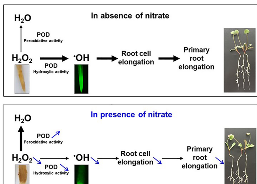
FIGURE 9 | ROS and POD govern primary root growth in M. truncatula . In absence of nitrate ( upper panel ), H 2 O 2 accumulated in the primary root tip is for a large part converted by POD hydroxylic activity in •OH, a ROS that favors root cell elongation, and root elongation, through cell wall polymer breaking. H 2 O 2 is also for a smaller part eliminated by POD peroxidative activity, resulting in H 2 O. In the presence of nitrate ( lower panel ), both the H 2 O 2 abundance and the POD hydroxylic activity decrease while POD peroxidative activity increases. As a result, •OH is less produced, restricting cell and root elongation. H 2 O 2 and •OH were detected in the root tip with diaminobenzidine (yellow color) and dihydrorhodamine (green fluorescence), respectively. 10-day old seedlings grown in the absence or the presence of 5 mM nitrate are presented at the right of the panels. Adapted from the graphical abstract of Zang et al. (2020).
