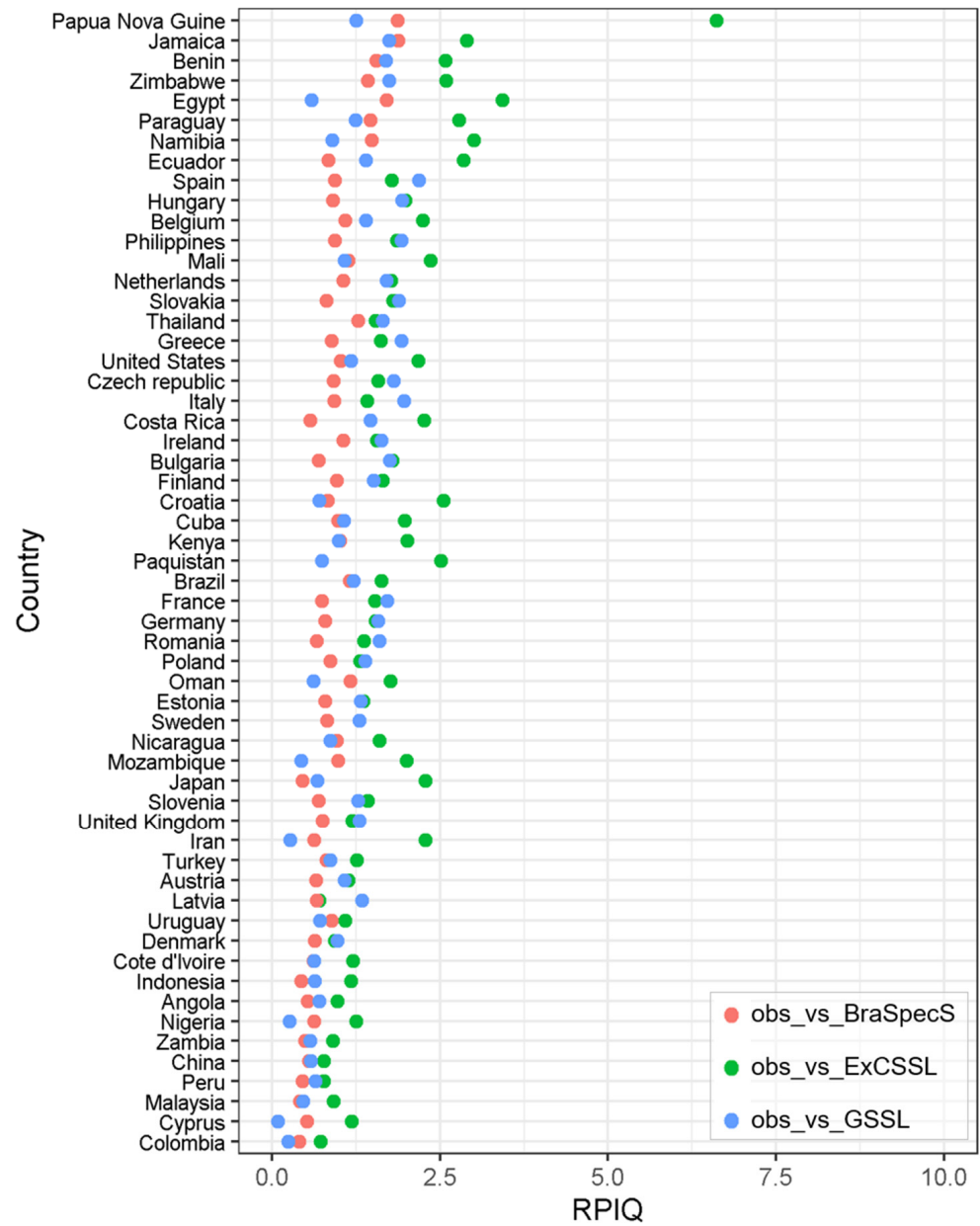
Figure 10. RPIQ for SOC models per country using vis-NIR-SWIR data.
