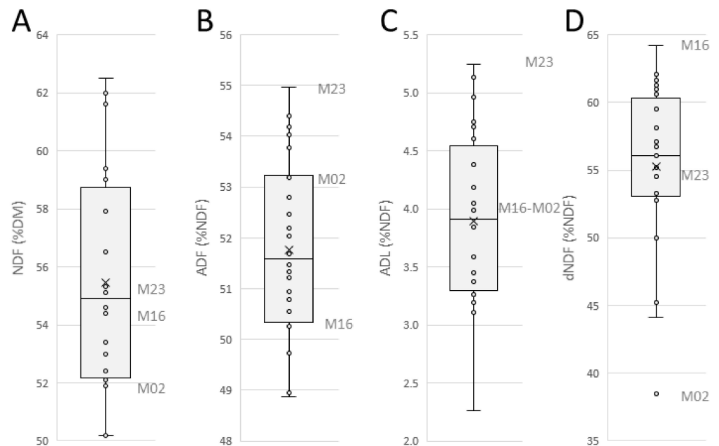
Figure 2. Fiber characteristics of 24 maize inbred lines of maize. (A) NDF = Neutral Detergent Fiber (% dm), (B) ADF = Acid Detergent Fiber (%NDF), (C) ADL = Acid Detergent Lignin (% NDF), (D) dNDF = digestibility of the NDF (% NDF).
