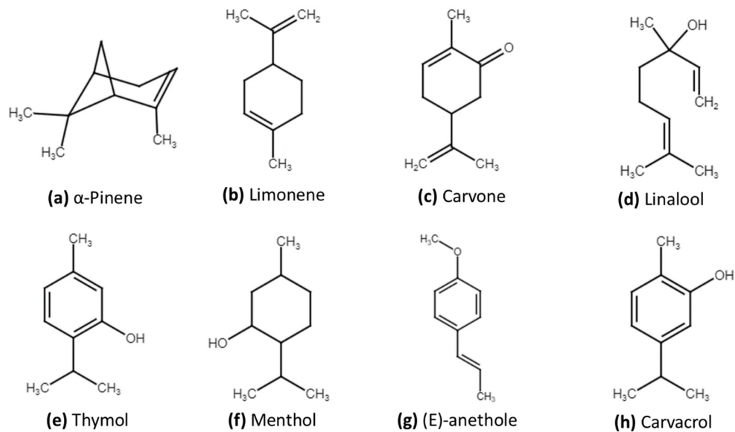
Figure 1. Chemical structure of several major components with potential biocidal activity;
