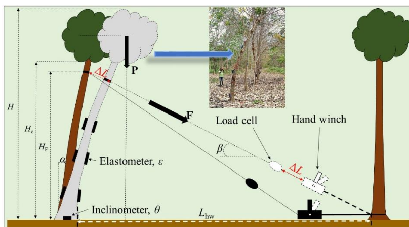
Figure 1: Principle of a trunk-bending test. H: total tree height; H c : crown-base height; H F : height of cable attachment to the tree; \alpha : initial inclination of tree base; \beta : cable angle; L hw : distance from tree base to cable anchorage; \epsilon : surface deformation; \theta : inclination of root-ground system; F : applied force; P : crown weight; \Delta L cable shortening.
