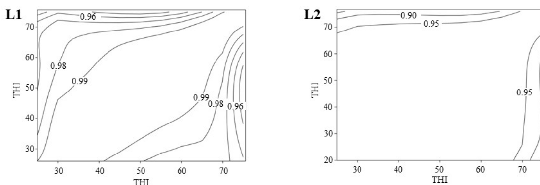
Figure 2. Genetic correlation estimates for MY at DIM 150d in L1 (left) and L2 (right) between all combinations of THI.
