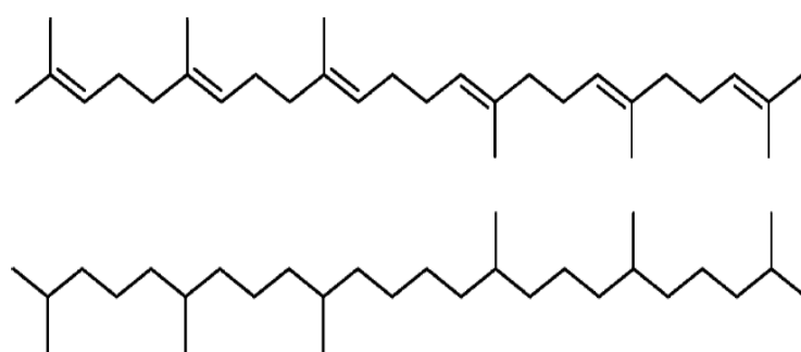
Figure 1. Chemical structure of squalene (top) and squalane (bottom).
