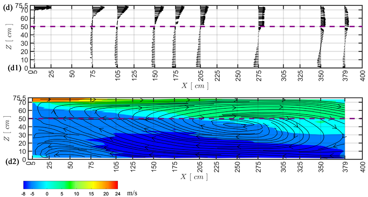
Figure 5. Comparison of the mean flow organization between configurations of empty enclosure and the three perforated plate cases: Z = 60.5 \text{ cm} - \phi = 0.3 , Z = 60.5 \text{ cm} - \phi = 0.5 and Z = 50.5 \text{ cm} - \phi = 0.5 . (a) Empty enclosure; (b) Perforated plate— Z = 60.5 \text{ cm} - \phi = 0.3 ; (b1) 2D velocity vectors using Laser-Doppler measurements (100 points); (b2) Streamlines superimposed with contour of longitudinal component of the velocity ( U ); (c) Perforated plate— Z = 60.5 \text{ cm} - \phi = 0.5 ; (c1) 2D velocity vectors using Laser-Doppler measurements (100 points); (c2) Streamlines superimposed with contour of longitudinal component of the velocity ( U ); (d) Perforated plate— Z = 50.5 \text{ cm} - \phi = 0.5 ; (d1) 2D velocity vectors using Laser-Doppler measurements (100 points); (d2) Streamlines superimposed with contour of longitudinal component of the velocity ( U ).
