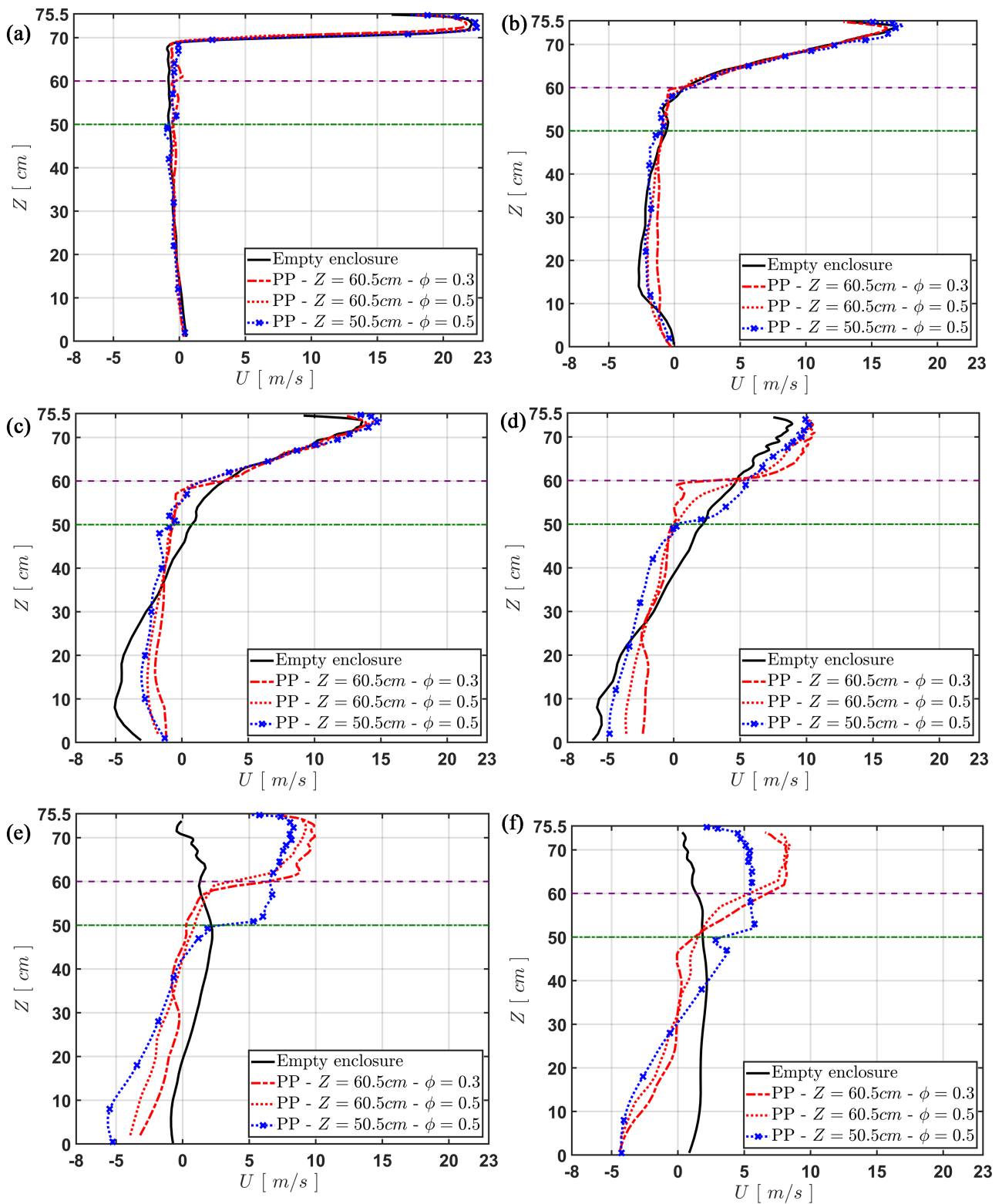
Figure 6. Effect of the perforated plate on the mean flow velocity profiles along the enclosure. (a) X = 5 cm ; (b) X = 75 cm ; (c) X = 105 cm ; (d) X = 205 cm ; (e) X = 275 cm ; (f) X = 350 cm .
