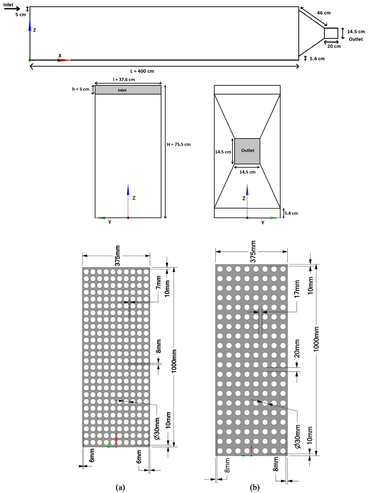
Figure 1. Schematic view of the empty enclosure and the perforated plates. (a) Perforated plate of thickness t = 4 mm and porosity of \phi = 0.5 ; (b) Perforated plate of thickness t = 4 mm and porosity of \phi = 0.3 .
