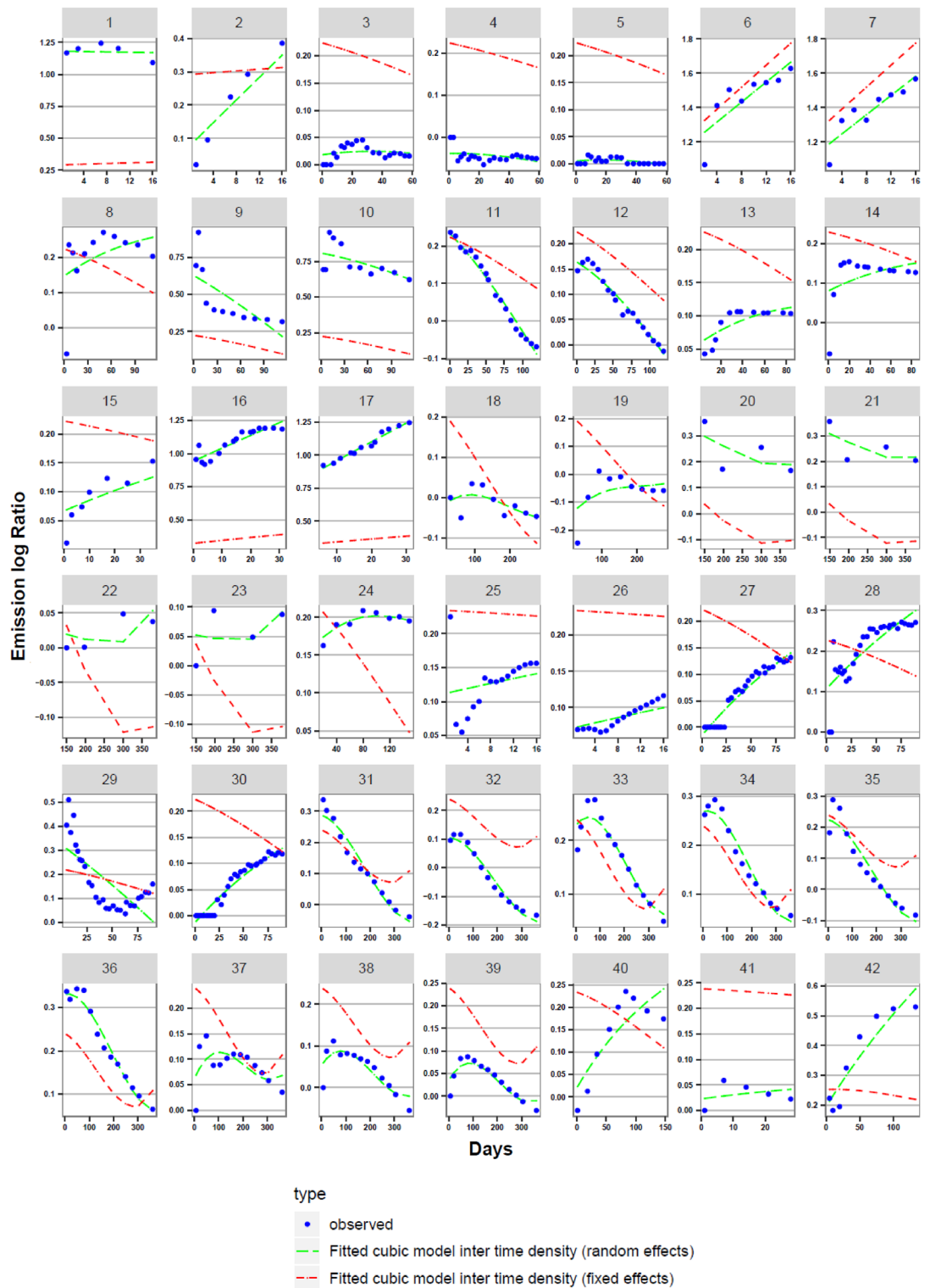
Figure 1. Evolution of the log ratio of CO 2 emissions with and without EW with time in the 42 experimental situations; comparison between experimental data (blue curve) and both mathematical models: one model with fixed temporal effects (red curve) and one model with the random temporal effects (green curve). The statistical parameters of both models are given in Table 2. The corresponding publication for each figure is: Figs. 1, 2 18 , Figs. 3–5 31 , Figs. 6, 7 32 , Figs. 8–10 7 , Figs. 11, 12 19 , Figs. 13, 14 33 , Fig. 15 30 , Figs. 16, 17 34 , Figs. 18, 19 27 , Figs. 20–23 22 , Fig. 24 35 , Figs. 25, 26 17 , Figs. 27–30 28 , Figs. 31–39 36 , Fig. 40 16 , Fig. 41 29 , Fig. 42 37 .
