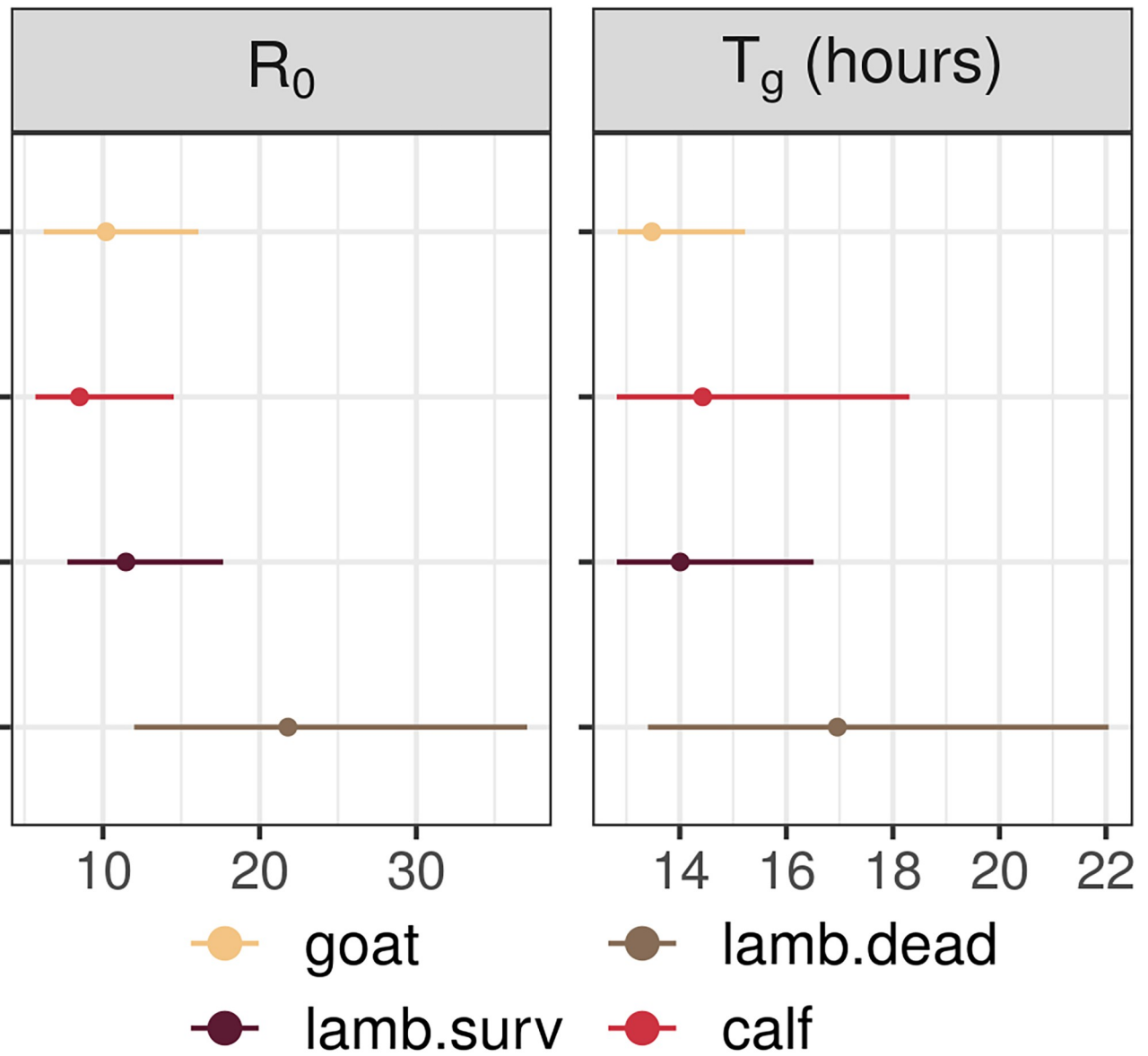
Fig 3. Outcome measures per host group. Points are median estimates, lines show highest density intervals, computed from joint posterior distributions (3 chains). Basic reproduction number R_0 is computed with Eq (3) and generation time T_g with Eq (4) . Note that generation times are constrained in their lower values due to the eclipse phase duration ( \kappa^{-1} ) and rate of virus entry into cells ( \beta ) being fixed ( Table 1 ).
