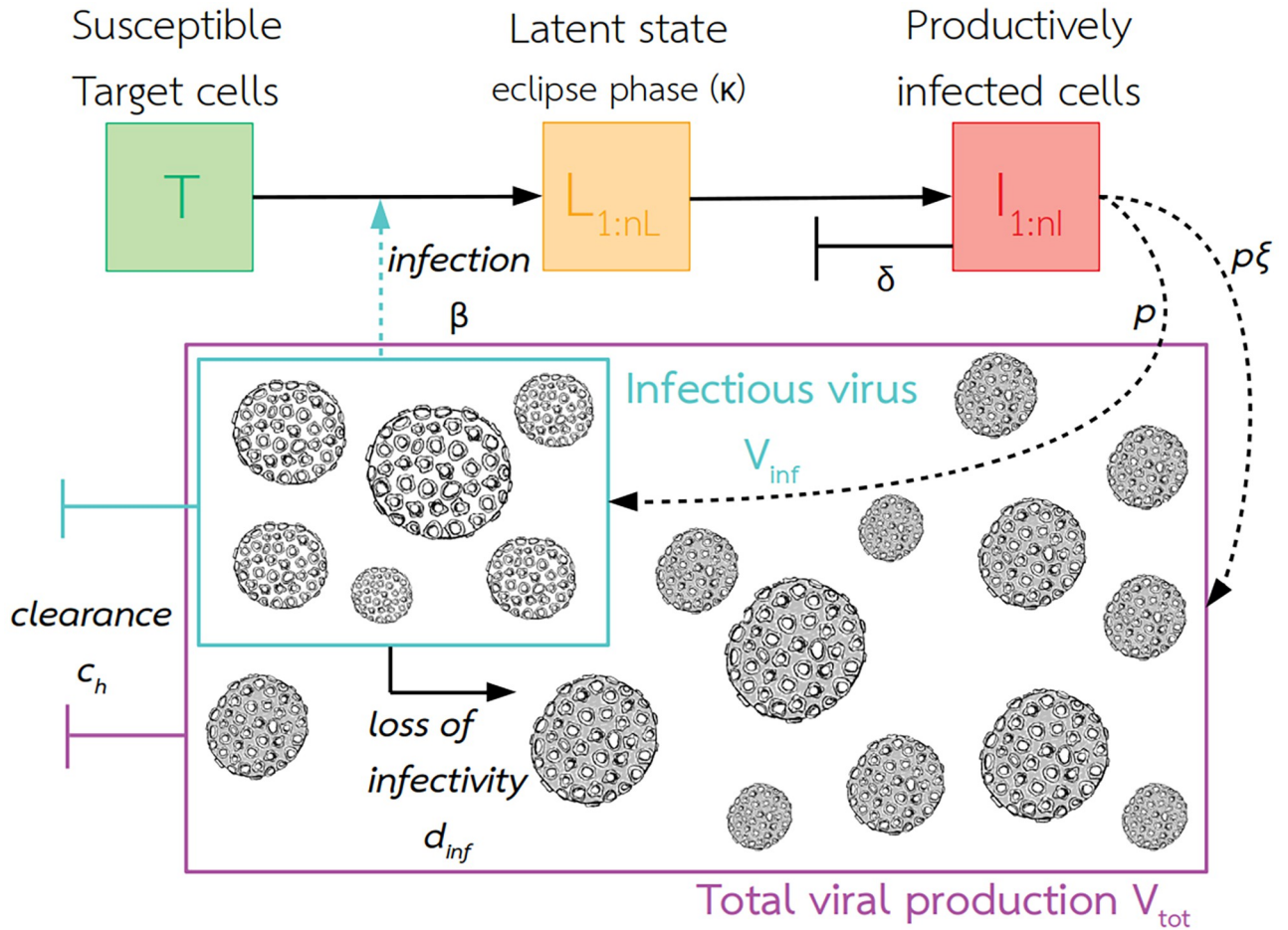
Fig 1. Graphical representation of the within-host model. Infectious viruses V_{inf} were fitted to TCID 50 measures, and total viral production V_{tot} to RT-qPCR measures. The eclipse phase (state L ) is the period between the infection of a cell by a virus and the presence of mature viruses within the cell. Productively infected cells I are the only ones producing progeny virions. Subscripts in L and I indicate the use of Erlang distributions for the time spent in those states. Target cells are not replenished and only productively infected cells die. Model assumptions, equations and parameter definitions can be found in Materials and methods, Eq (1), and Table 1.
