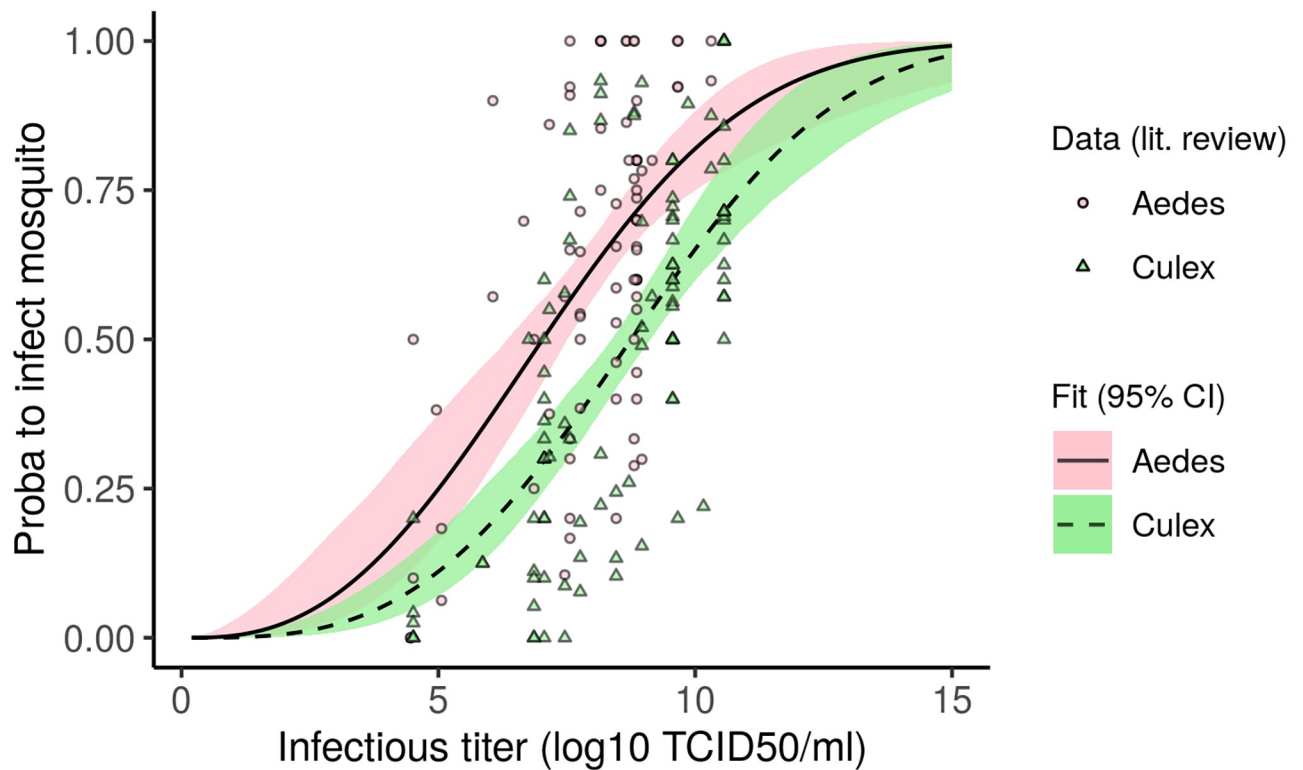
Fig 4. Dose-response relationships linking host infectious titers to the probability to infect mosquito vectors. Data retrieved from a systematic review (Materials and methods, Section S.2.1 in S1 Text). Points and triangles show infection rates (presence of RVFV in mosquito bodies, legs excluded) from experiments performed with hamsters with RVFV strain ZH501. Fits were obtained with Eq (S.6) in S1 Text using a betabinomial likelihood to account for overdispersal in the data. Confidence intervals result from 1000 replicate trajectories. Note that infectious titers >10 \log_{10} TCID 50 /ml are not to be expected in hosts, but were included to show the full curve.
