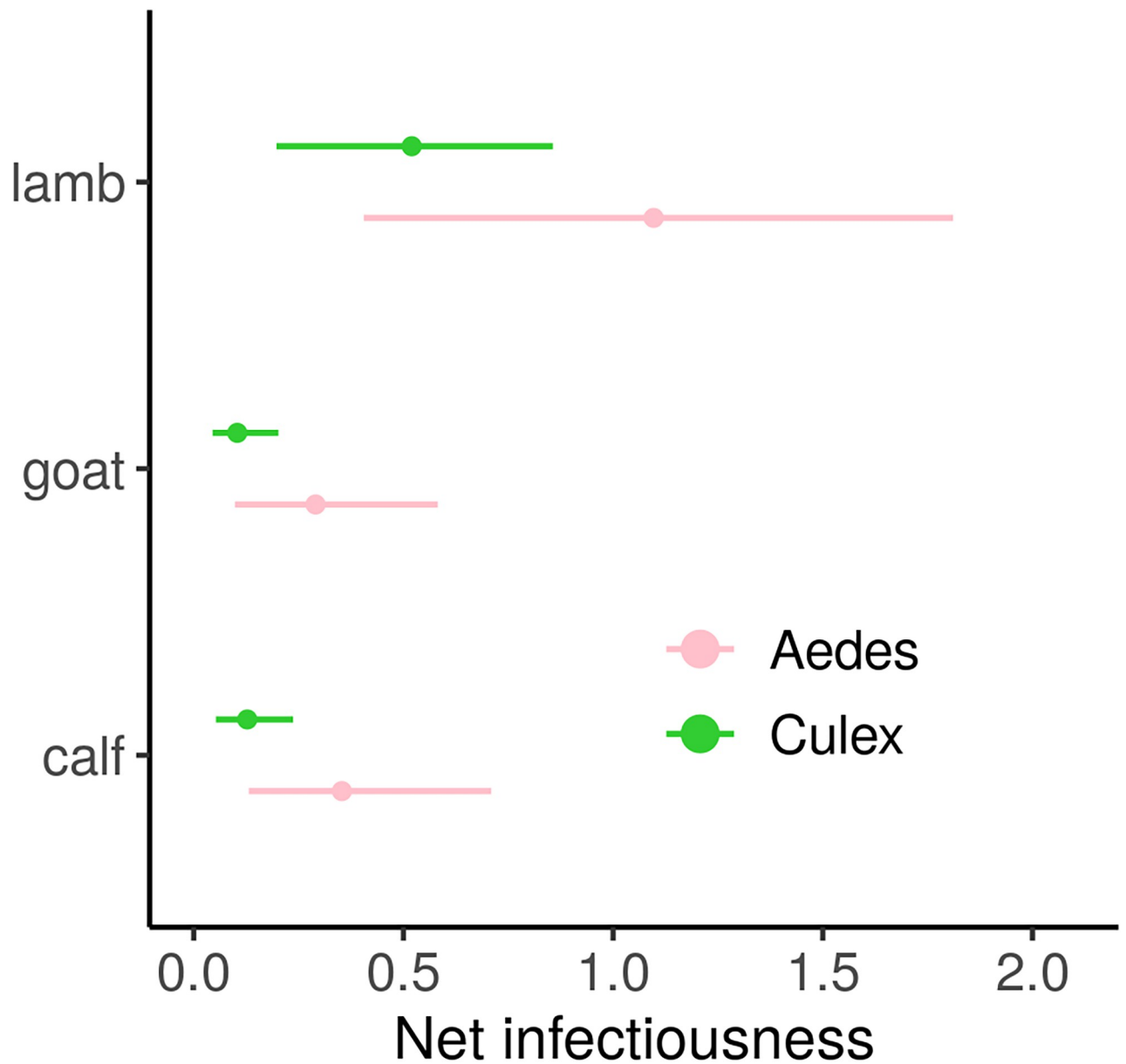
Fig 5. Net infectiousness of RVFV livestock host species, function of the mosquito genus involved in transmission. Points are median estimates, lines show highest density intervals, computed using 1000 parameter sets from the within-host model and dose-response curve respective fitting procedures. For lambs, parameters were sampled in the posteriors of both surviving and dying groups, according to the survival rate observed in the original dataset (6/16, Fig H in S1 Text). Time of death also varied according to a Weibull survival model (Materials and methods).
