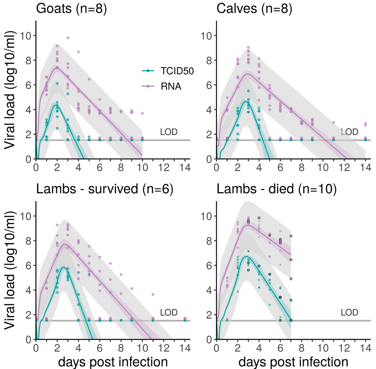
Fig 2. Data on viral RNA (RT-qPCR) and infectious virus (TCID 50 ), in log 10 /ml of plasma, and model fits, for host groups showing significantly different viral dynamics. Circles are data points. Solid colored lines show the median fit, obtained from 1000 posterior draws. Inner envelopes using the same colors shows the uncertainty from the parameter estimation process (quantiles [2.5–97.5]% of these posterior draws). Outer grey envelopes show the 95% uncertainty bounds associated with the observation process. We assumed this to be normally distributed with a standard deviation of 1 (log 10 scale), in line with the sampling error. Purple is for viral RNA and blue for infectious viruses. For lambs which died from RVF, circled points represent individuals' time of death. LOD = limit of detection, 1.55 for TCID 50 , 1.7 for viral RNA (log 10 ).
