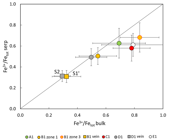
Fig. 11. \text{Fe}^{3+}/\text{Fe}_{\text{tot}} ratio of serpentine plotted versus bulk \text{Fe}^{3+}/\text{Fe}_{\text{tot}} ratio of sample.
