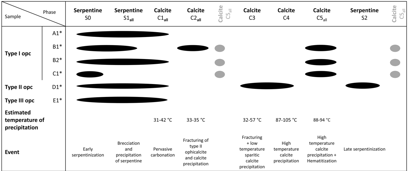
Fig. 13. Relative chronology of the different episodes of alteration. In grey color, are the possible scenarios for calcite C5 all .
