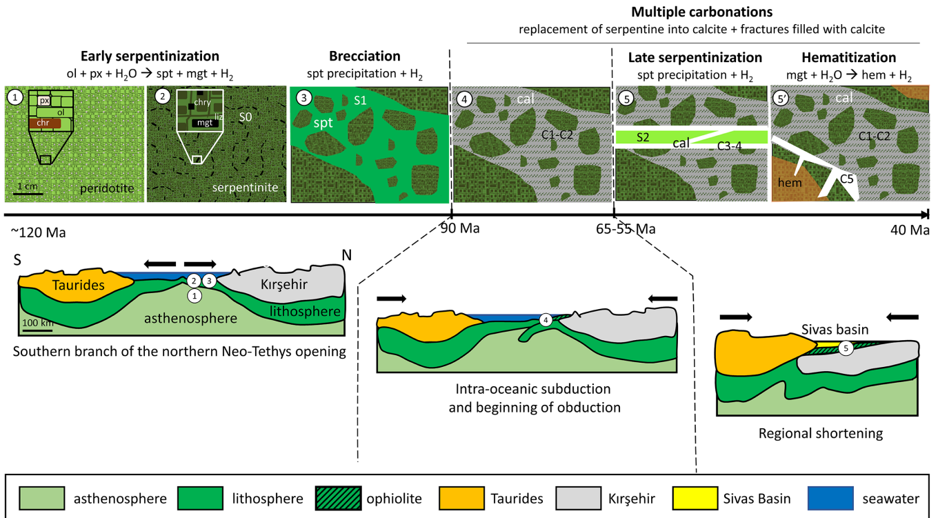
Fig. 14. Sketch of the different alteration events from the seafloor to the continent. cal: calcite; chr: chromite; chry: chrysotile; hem: hematite; liz: lizardite; mgt: magnetite; ol: olivine; px: pyroxene; spt: serpentine.
