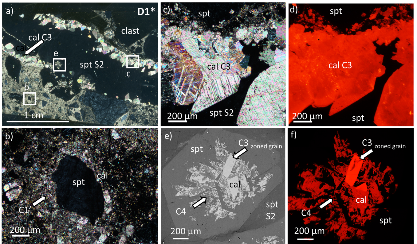
Fig. 8. (a) XPL image of D1* and (b) magnified view of the partially carbonated clast; (c) euhedral grains of calcite at the border of the S2 serpentinite with (d) the associated cathodoluminescence image; (e) a grain of serpentinite with euhedral and dendritic calcite at the border of the S2 serpentinite with (f) the associated cathodoluminescence image. cal: calcite; spt: serpentinite.
