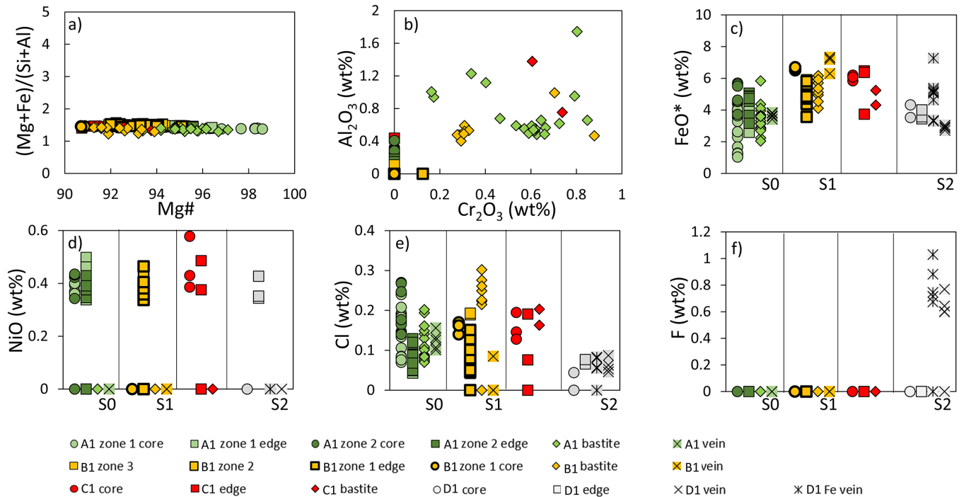
Fig. 10. Chemical compositions of the serpentines. (a) (\text{Mg} + \text{Fe})/(\text{Si} + \text{Al}) ratio versus \text{Mg}/(\text{Mg} + \text{Fe}) noted as Mg#. (b) \text{Al}_2\text{O}_3 oxides versus \text{Cr}_2\text{O}_3 . The bastites are enriched in those oxides compared to the serpentines replacing olivine. (c–f) Abundances of \text{FeO}^* , NiO, Cl and F. When a value was below the detection limit of an element, it was set to 0, which explains the basal trends.
