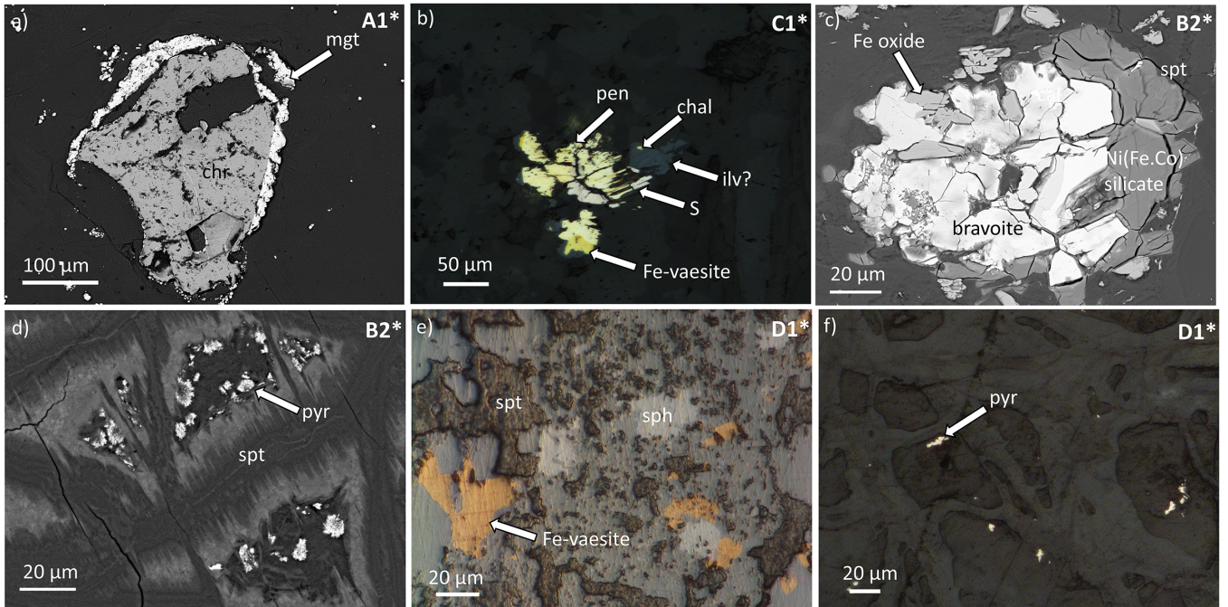
Fig. 7. (a) A chromite grain bordered with magnetite from A1*. (b) Image in reflection of opaque minerals in B2*. (c) SEM image of a bravoite grain bordered by Ni(Fe,Co) silicate and Fe oxide in B2*. (d) SEM image of pyrite present in cores of the mesh of serpentinite in B2*. (e) Image in reflection of Fe-vaesite and sphalerite and (f) some pyrite present in the cores of the mesh of serpentinite clasts in D1*. cal: calcite; chal: chalcopyrite; chr: chromite; ilv: ilvaite; mgt: magnetite; pen: pentlandite; pyr: pyrite; sph: sphalerite; spt: serpentinite.
