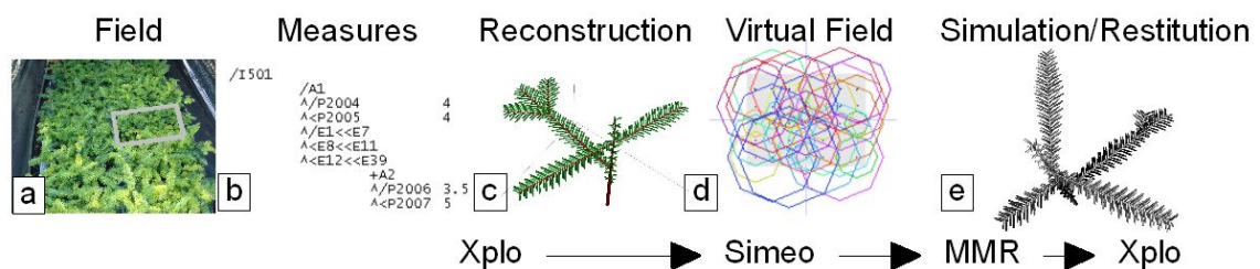
Figure 2: From plot to simulation , (a) view of a subplot in the dry (D) treatment, (b) plant architecture coded in accordance with AMAPMOD/MTG syntax (Godin & Caraglio, 1998), (c) topological and geometrical plant reconstruction with Xplo, (d) stand reconstruction with Simeo, (e) light interception calculated using MMR model and analyses by Xplo.
