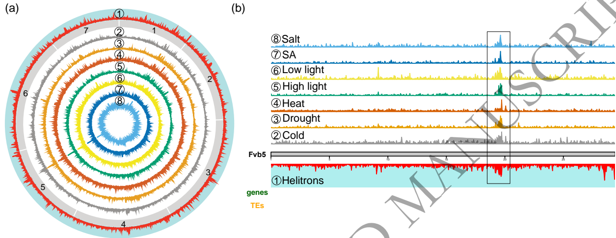
Fig. 6 Genome-Wide distribution of DMR densities. (a) Circa plot showing DMR densities on all 7 strawberry chromosomes (gray boxes) for each stress condition (2. Cold, 3. Drought, 4. Heat, 5. High light, 6. Low light, 7. SA, and 8. Salt). Helitron density (1) in the genome is depicted on the outer most circle in red with turquoise background. (b) DMR density depicted on chromosome 5 (Fvb5) displaying a common enrichment among all the stress conditions (left of the 20 Mb tick mark). Below, the chromosome is indicated in grey, green shows gene density, yellow the TE density and red Helitrons along the chromosome.
