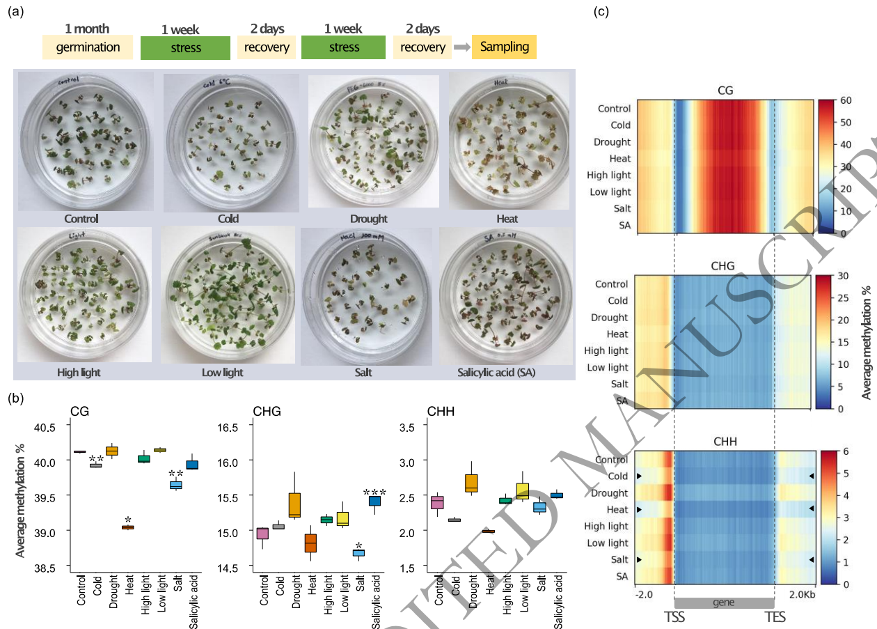
Fig. 1 Effect of abiotic and hormone stresses on genome-wide DNA methylation levels in F. vesca . (a) Top: Scheme of stress treatment time course. Bottom: Photographs of plates with one-month-old plants grown under different stress conditions (cold, drought, heat, high and low intensity of light, salt, and salicylic acid). (b) Average DNA methylation levels for each cytosine context (CG, CHG, CHH) between normal and stress conditions (only common cytosines positions among all samples were considered that had a minimum coverage of 5 reads). Asterisks indicate levels of significance between treated and control plants: *, p-value < 0.05; **, p-value < 0.01; ***, p-value < 0.001 (unpaired two-tailed Student's t-test). (c) Heat maps showing distribution of DNA methylation (top: CG, middle: CHG, and bottom: CHH context) around genes with and without stress (Control). Mean of the average methylation percentage (within a sliding 100-bp window) was plotted 2 kb upstream of TSS, over the gene body and 2 kb downstream of TES. Black arrows highlight the samples in which a reduction of DNA methylation can be observed in the vicinity of TSS and TES sites.
