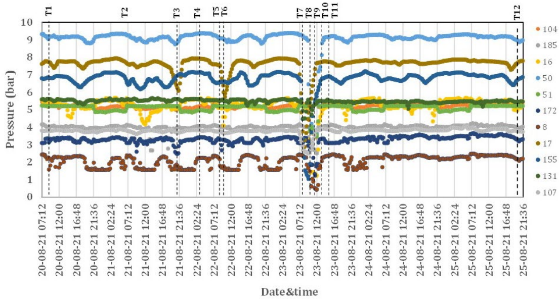
Figure 3. Pressure history from the working sensors for Example 1
