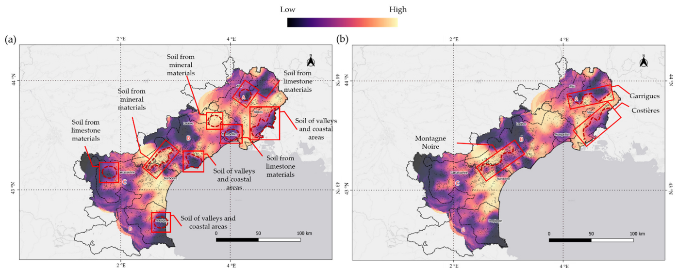
Figure 7. The interpolated 2020 Co1 map overlaid with summary information (Table 5) that was identified by multiple experts and associated with effects attributed to: (a) the variation in the pedological units and (b) the variation in the geological units for 2020 made by the group of experts for each sector. Light colours represent high score values and dark colours represent low score values for Co1. Areas of the experts' observations are highlighted in red squares.
