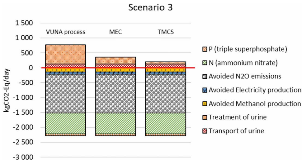
Figure 6 | Comparison of greenhouse gases emissions for the three different treatment technologies (VUNA process, microbial electrolysis cell (MEC), and transmembrane chemisorption (TMCS), for the Scenario 3. Comparison for the two other scenarios is given in supplementary information (Table S4).
