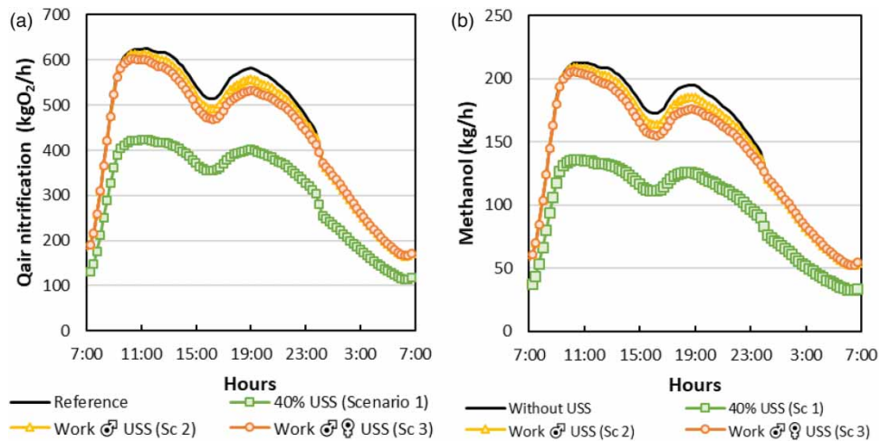
Figure 5 | Daily aeration flow needed at the biofilters to achieve nitrification, (a) and daily methanol dosing required to achieve post denitrification (b) for the reference and the three urine retention scenarios.
