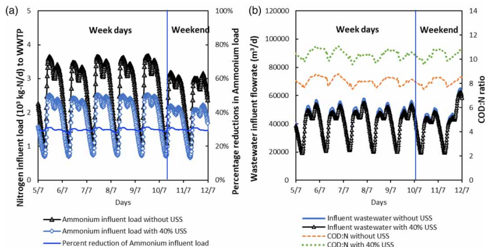
Figure 2 | (a) Flows of ammonium influent loads ( 10^3 \text{ kgN/d} ) and the percentage of reduction in ammonium influent at the WWTP; (b) Wastewater influent flowrates ( \text{m}^3/\text{d} ) along with the COD:N ratios, without urine source separation (USS) and with 40% USS rate, for the MAV plant and for scenario 1 (S1).
