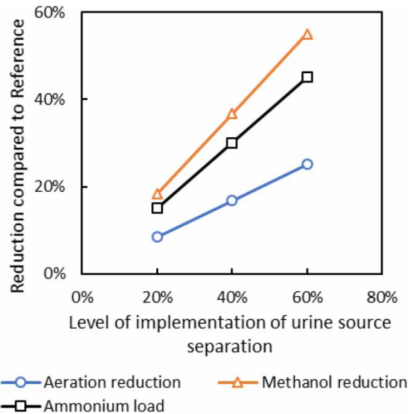
Figure 3 | Comparison of reduction need of methanol, aeration and ammonium load entering the wastewater treatment plant, for scenarios with 20, 40 and 60% urine separation rate.
