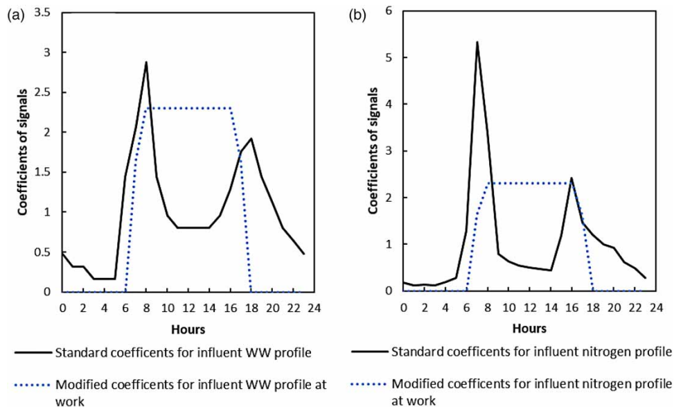
Figure 1 | Standard and modified coefficients for wastewater profile generation (a) and for nitrogen production (b), which simulates urine generating profiles. Normal profile production are typically characterized by a morning peak production around 8:00 a.m. and another peak production in the afternoon, around 6:00 p.m. The modified profile generation target production during working hours only, between 8:00 a.m. and 5:00 p.m.
