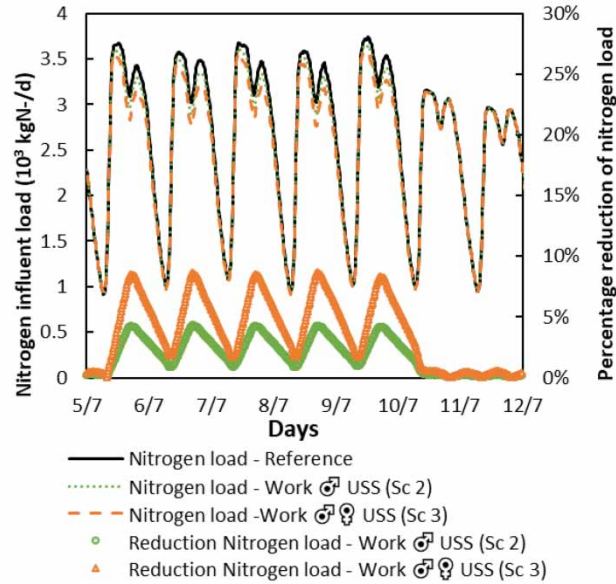
Figure 4 | Nitrogen influent load for MAV Plant for reference scenario (without USS) and for urine source separation scenarios 2 (men urinals) and 3 (all toilets) at work and their corresponding percentage reduction in nitrogen influent load.
