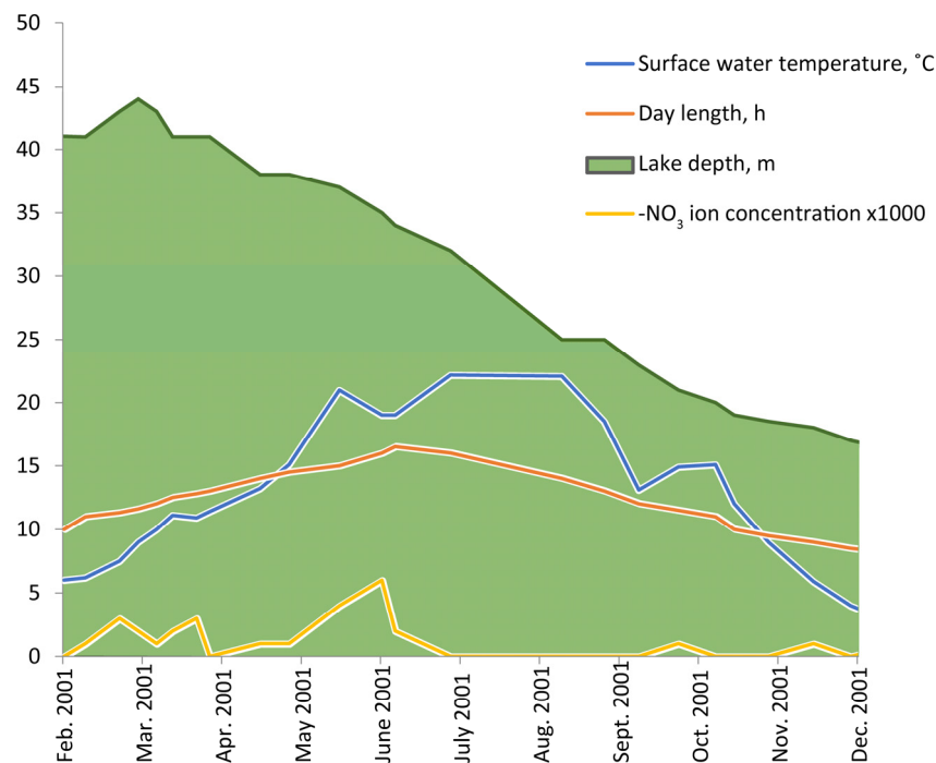
Figure 1. Abiotic parameters evolution in Lake Grand Laouicien in 2001.
