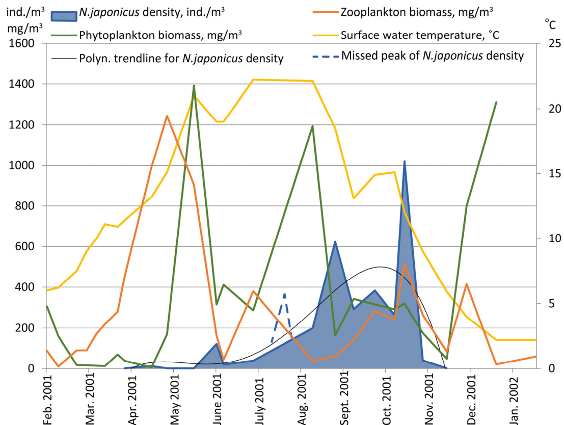
Figure 2. Seasonal dynamics of phyto- and zooplankton biomasses and Neogasilus japonicus population density in Lake Grand Laoucien, 2001.
