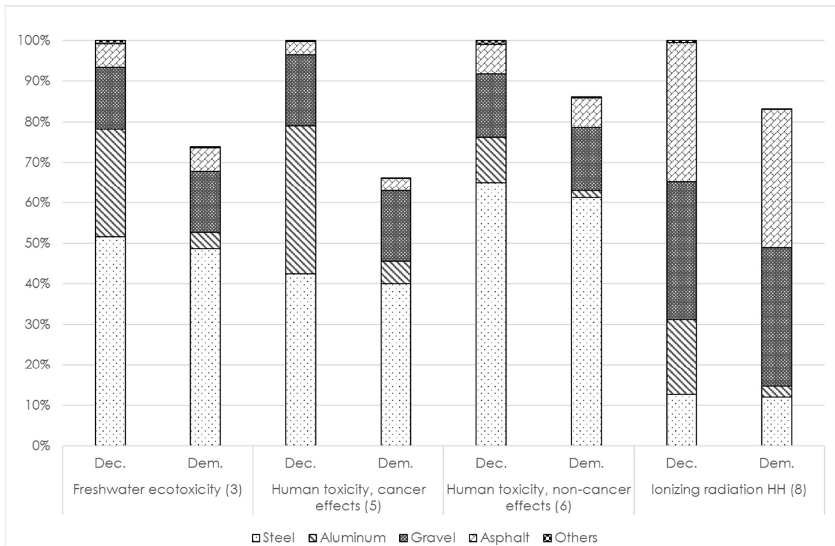
Figure 5 : Product type contribution on several environmental impacts of stage D for an exhibition hall deconstruction (Dec.) and the demolition alternative scenario (Dem.)
