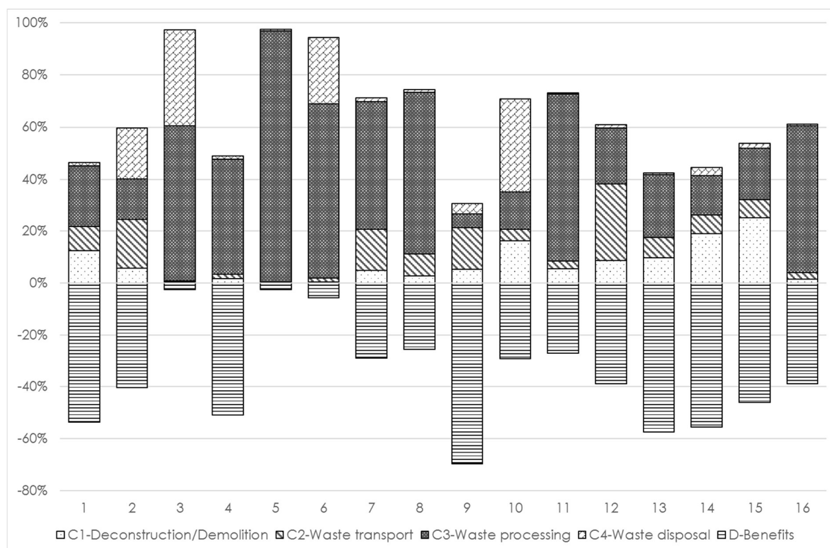
Figure 2 : Contribution of building end-of-life stages on environmental impacts for deconstruction of an exhibition hall – the impacts numbering is in Table 6
