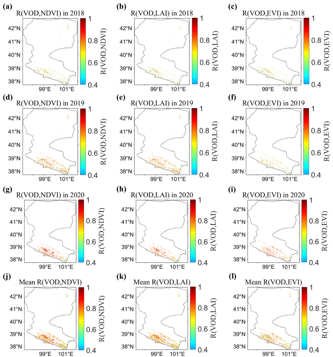
Figure 10. The correlation coefficient (R) between VOD (from top to bottom: VOD in 2018 (a–c), VOD in 2019 (d–f), VOD in 2020 (g–i), the three yearly average VOD (j–l)) and three MODIS VIs (from left to right: NDVI, LAI, EVI).
