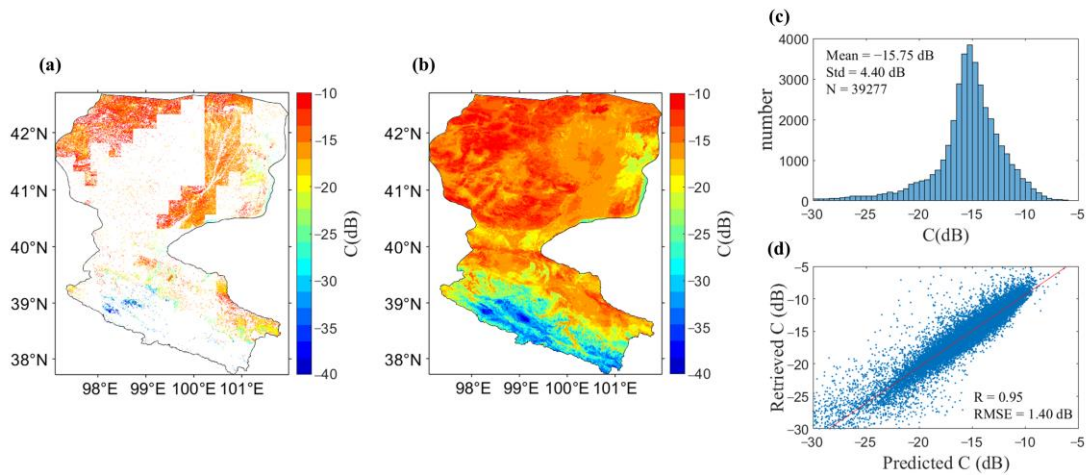
Figure 3. The computation results of the C values in 2018. (a) Map of the retrieved soil parameters; (b) map of the RF predicted C soil parameters; (c) histograms of the retrieved C, and (d) scatterplot between the retrieved and RF predicted values for the C value.
