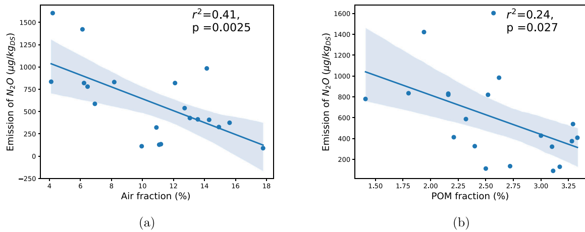
Fig. 7. Air (a) and POM (b) fractions per soil core as a function of the accumulated N_2O emission during the seventh day, with their respective tendency line. The shaded area corresponds to the 95% confidence interval band for the fitted slope and intercept (which implies a 95% chance that the true regression line fits within the confidence bands).
