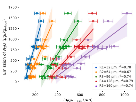
Fig. 10. \text{N}_2\text{O} emissions at day 7 in function of the descriptors Id_{\text{POM-air}} . Each of them present its linear regression along with a translucent 95% confidence interval band.
