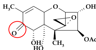
Figure 1: Chemical structures of trichothecenes. Dietary TCTs are classified in two main groups. Group A TCTs include T-2 toxin (T-2), diacetoxyscirpenol (DAS), and NX. Group B TCTs include deoxynivalenol (DON), nivalenol (NIV), and fusarenon-X (FX). Group A TCTs can be distinguished from group B TCTs by the presence of a C 8 keto-oxygen (circled in red).
