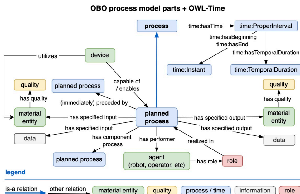
Fig. 11: OBO + OWL-time process modelling. Inputs and outputs can have qualities (or characteristics) attached to them which can change from input to output.
