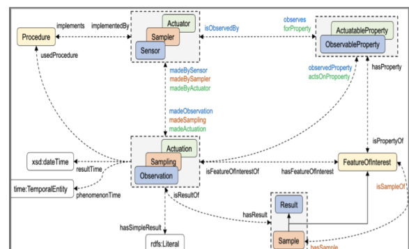
Fig. 15: The SOSA model. CREDIT: (sent request to https://www.researchgate.net/publication/325644558 ).
