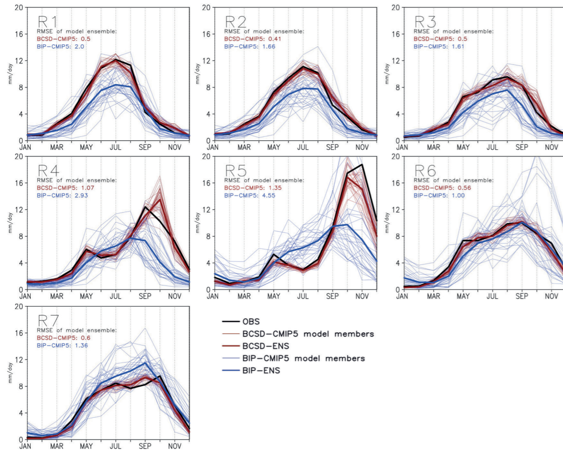
[ Figure 1.6 ] Seasonal precipitation cycles for the seven climatic sub-regions for the period 1996–2005
