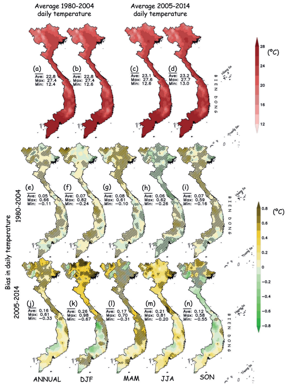
Spatial distribution of the average temperature in Viet Nam according to OBS and CMIP6-ENS; (a, b) and (c, d) indicate the average temperature of 1980–2004 and 2005–2014 by OBS and CMIP6-ENS, respectively; (e-i) and (j-k) show the biases of CMIP6-ENS compared to OBS for the training period 1980–2004 and the testing period 2005–2014. The hatched lines show the regions in which more than two-thirds CMIP6 models have the same sign as BCSD-ENS. Figure modified from Tran-Anh et al. (2022b).
