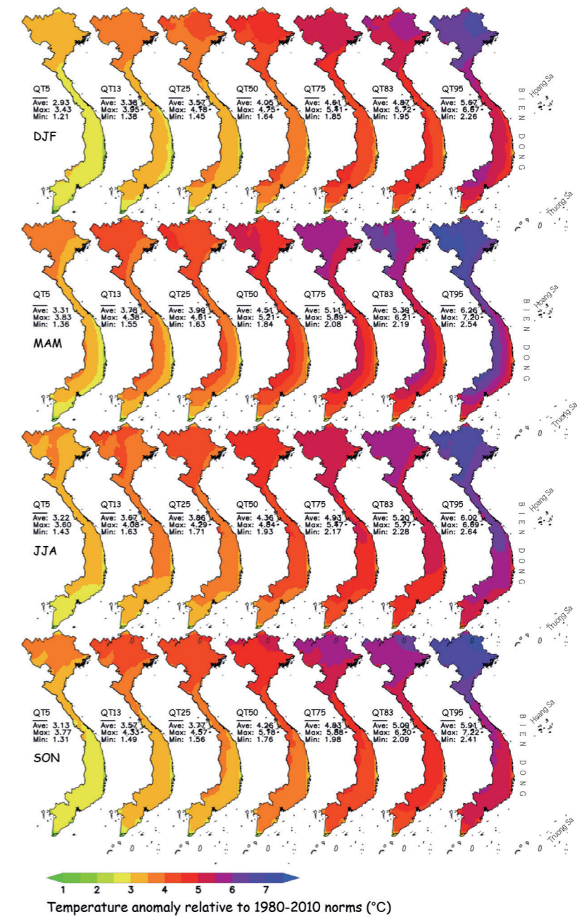
[ Figure 1.19 ] Average seasonal temperature anomaly in 2080–2099 relative to the 1980–2010 period under SSP5-8.5
