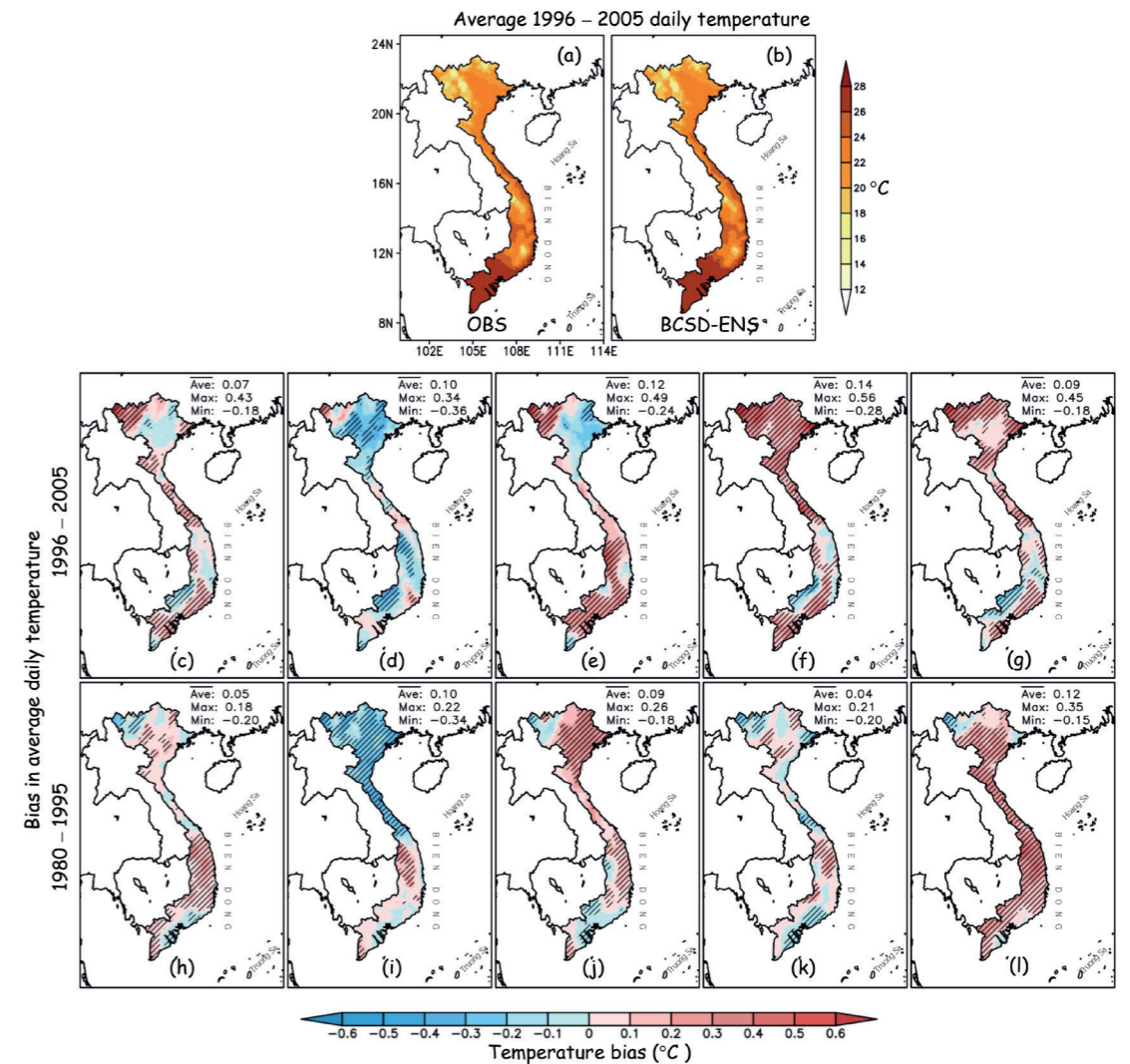
Spatial distribution of average temperature and biases in Viet Nam
