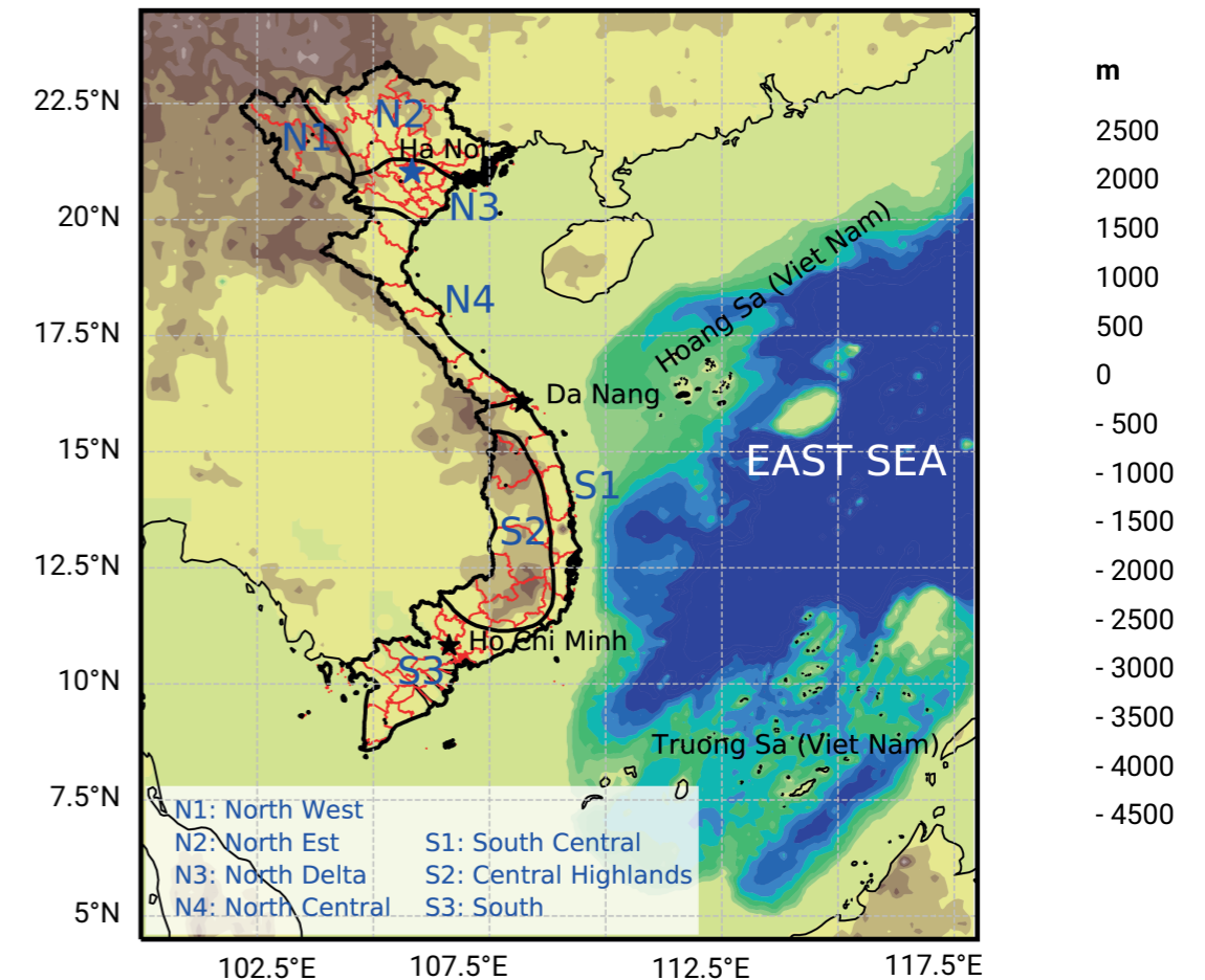
[Figure 1.1] Topography of Viet Nam and surrounding areas
