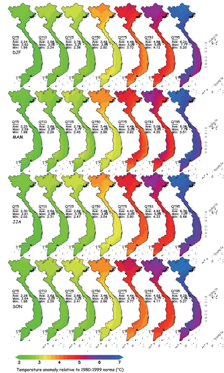
[Figure 1.17] Average seasonal temperature anomaly in 2080–2099 relative to the 1980–1999 period under RCP8.5
