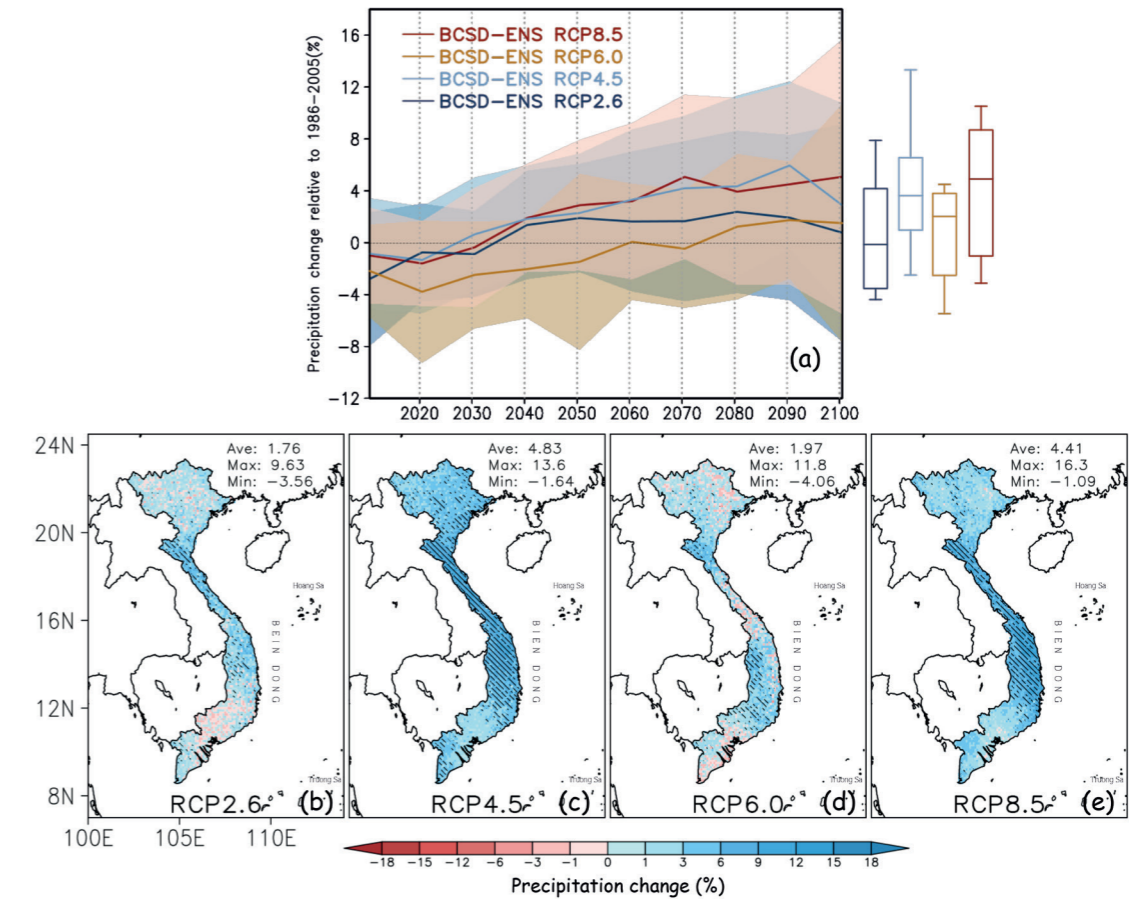
[Figure 1.13] Projected precipitation changes in Viet Nam under different RCPs
