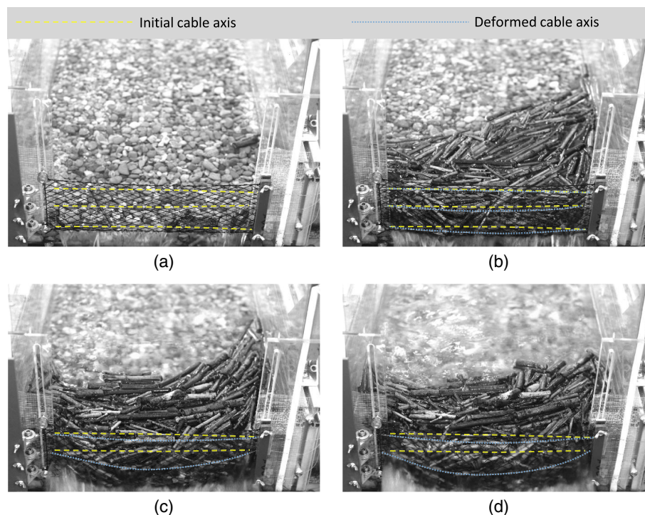
Fig. 7. Pictures of the progressive deformation of the net and the sensor cables (highlighted in color: yellow for initial position and blue for deformed position). The bottom cable being hidden by water jets and logs is not visible for the pictures (c and d) and thus not highlighted: (a) 14:28 ( Q = 1 l/s); (b) 14:34 ( Q = 2 l/s); (c) 14:46 ( Q = 5 l/s); and (d) 14:58 ( Q = 7.6 l/s).
