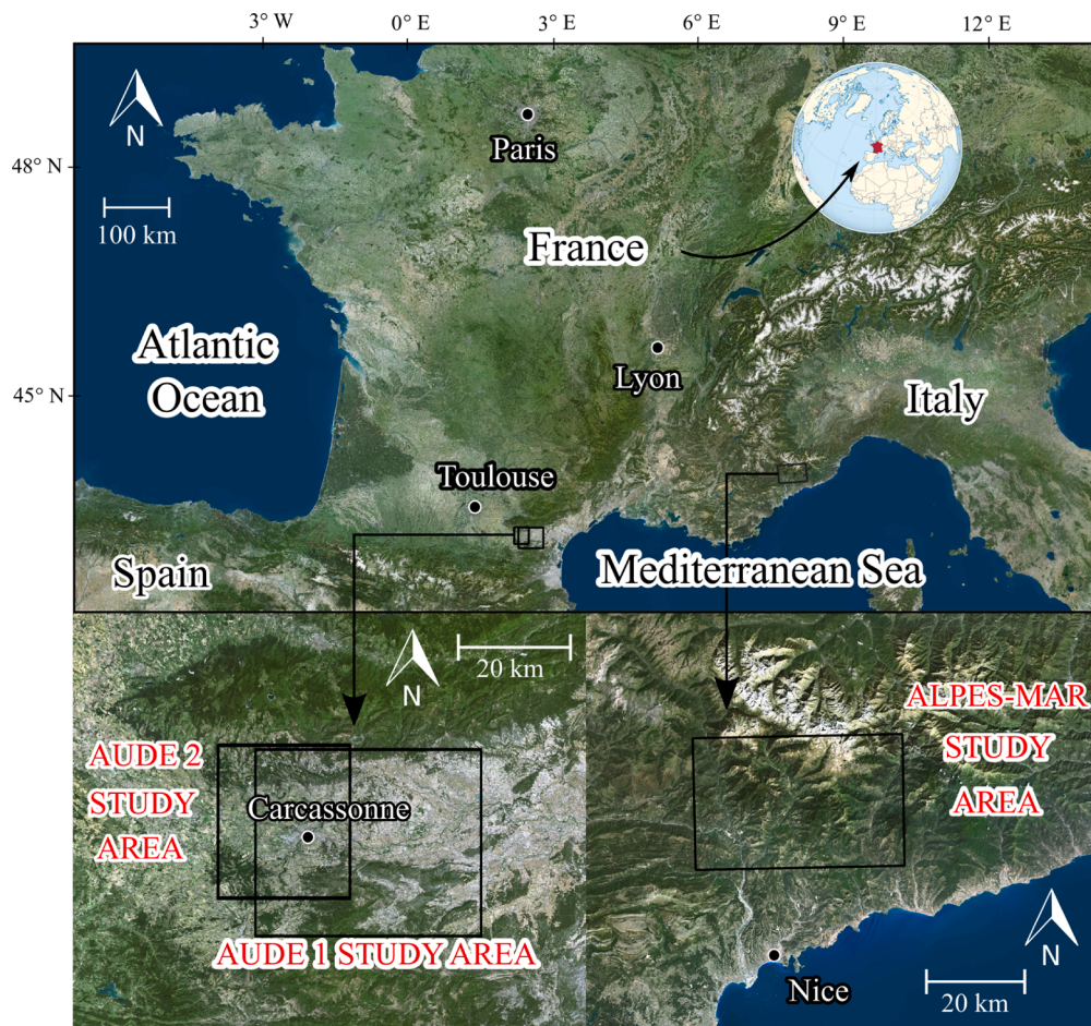
Fig. 1. Study areas in Aude and Alpes-Maritimes departments, France (IGN airborne orthophotos, 2017).
