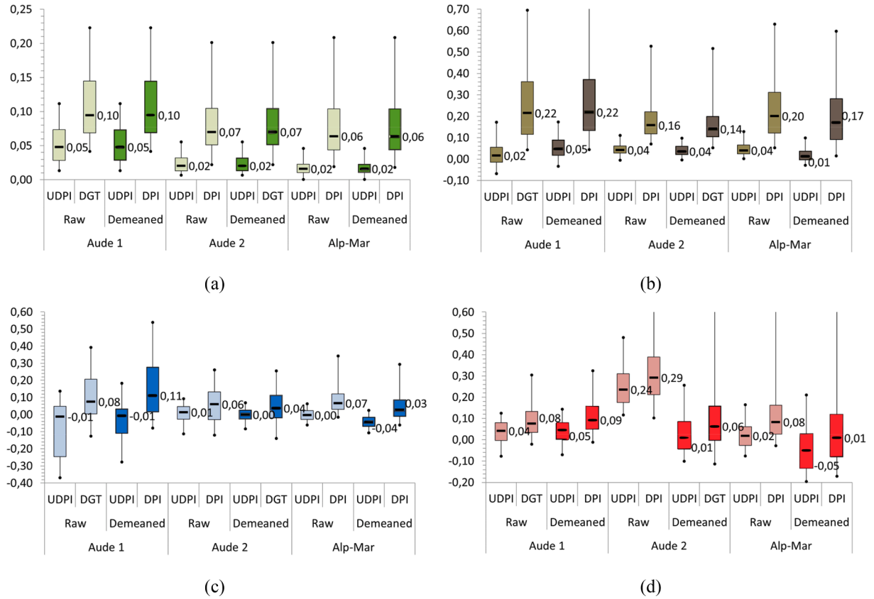
Fig. 9. Boxplot of (RD^k)_\theta distributions (raw and with land use demeaning pre-processing) based on the closest S2 and S1 change images. (a) k = NDVI , \theta = \text{standard deviation} ; (b) k = NDWI , \theta = \text{maximum} ; (c) k = SAVI , \theta = \text{mean} ; (d) k = VV polarization when NDVI < 0.25 , \theta = \text{maximum} .
