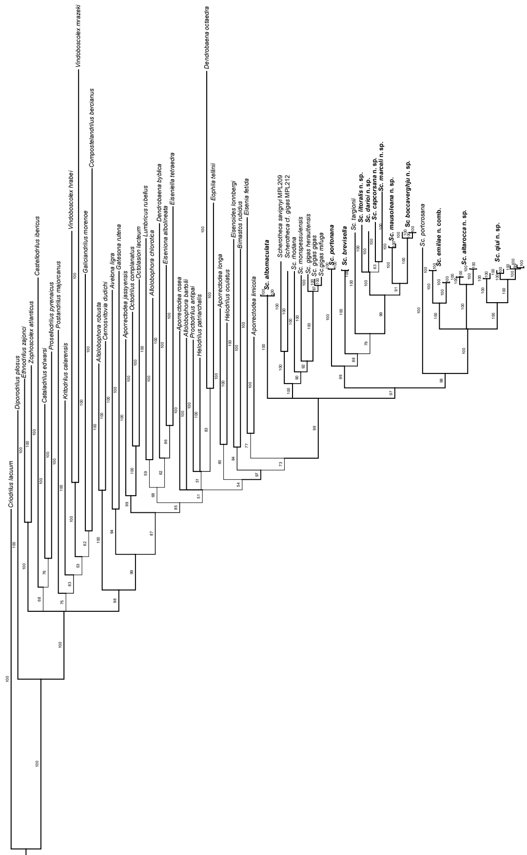
APPENDIX 3. — Phylogenetic tree obtained by Bayesian phylogenetic analysis of the concatenated sequence of molecular markers COI, 16S, ND1, and 28S. The species sequenced in this work are shown in bold. Posterior probability support values are shown above the corresponding branches.
